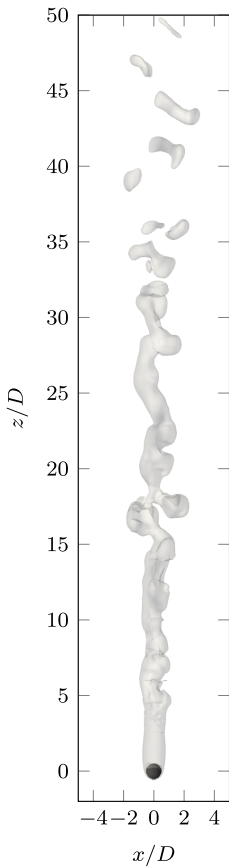
(b) Re = 600
