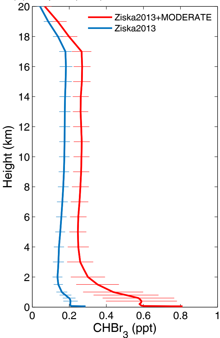
(a) Tropics (DJF)
