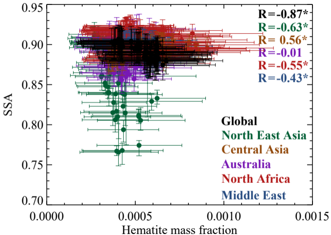
(a) Aitken+accumulation
