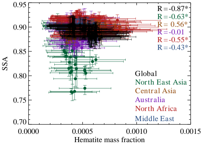
Aitken+accumulation
