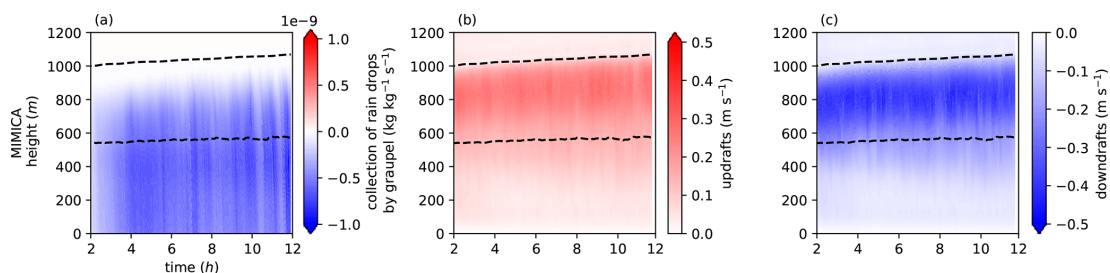
Figure A8. (a) Collection of raindrops by graupel, (b) updrafts and (c) downdrafts with time, as simulated by MIMICA. The first 2 h of simulations, considered as the spin-up period, are excluded. For figure clarity, the plot titles have been abbreviated; the first number refers to the accumulation mode and the second to the Aitken mode concentration in cubic centimetres, i.e. 3_20 refers to AC3_AK20. Black dashed lines represent the cloud top and cloud base heights.
