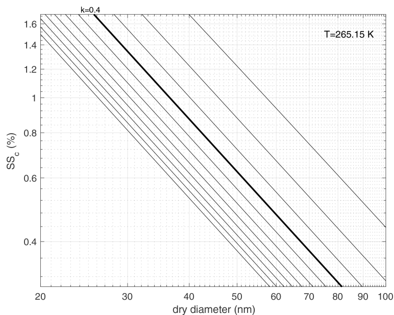
Figure A12. Calculated critical supersaturations SS_c (in percent) as a function of dry diameter, computed for \sigma_s/a = 0.072 \text{ J m}^{-2} and T = 265.15 \text{ K} . \kappa lines are shown for a range 0.1 \leq \kappa \leq 1.1 . Bold line corresponds to \kappa = 0.4 .
