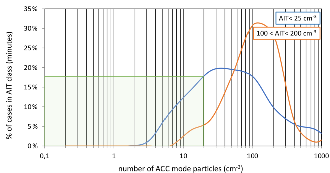
Figure 16. The occurrence probability (percent of total minutes of observations) for two classes of Aitken (AIT) mode concentrations, i.e. \text{AIT} < 25 \text{ cm}^{-3} and 100 < \text{AIT} < 200 \text{ cm}^{-3} . On the x axis is the number of accumulation (ACC) mode particles in cubic centimetres. The statistics are calculated for four different expeditions in the high Arctic in the summers of 1991, 1996, 2001 and 2008. Further details on the quality and data processing of the aerosol size resolved measurements are available in Heintzenberg and Leck (2012).
