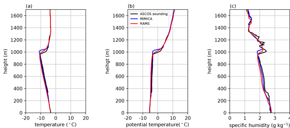
Figure 1. Radiosonde observations from 05:35 UTC on 31 August 2008 of (a) absolute temperature, (b) potential temperature and (c) specific humidity. The corresponding simulated profiles from MIMICA and RAMS are presented for the middle of the simulation period (6 h of simulation time).
