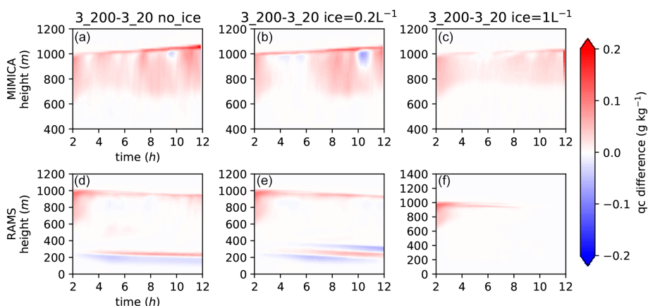
Figure 11. Differences in cloud water mixing ratio ( q_c ) for simulation pairs with the same accumulation mode concentration and the same ice crystal concentration equal to 0\text{ L}^{-1} (no_ice; a , d ), 0.2\text{ L}^{-1} ( b , e ) and 1\text{ L}^{-1} ( c , f ), shown for MIMICA and RAMS. The first 2 h of simulations, considered as the spin-up period, are excluded. A Student's t test with a 95 % confidence level shows that the (time mean) differences are statistically significantly different for each pair of simulations. For figure clarity, the plot titles have been abbreviated; the first number refers to the accumulation mode and the second to the Aitken mode concentration in cubic centimetres, i.e. 3_20 refers to AC3_AK20.
