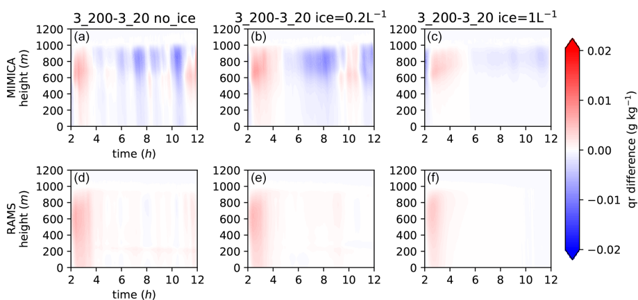
Figure 12. Differences in rain water mixing ratio ( q_r ) for simulation pairs with the same accumulation mode concentration and the same ice crystal concentration equal to 0\text{ L}^{-1} (no_ice; a , d ), 0.2\text{ L}^{-1} ( b , e ) and 1\text{ L}^{-1} ( c , f ), shown for MIMICA and RAMS. The first 2 h of simulations, considered as the spin-up period, are excluded. A Student's t test with a 95 % confidence level shows that the (time mean) differences are statistically significantly different for each pair of simulations except for the pair with ice crystal concentration of 1\text{ L}^{-1} in RAMS. For figure clarity, the plot titles have been abbreviated; the first number refers to the accumulation mode and the second to the Aitken mode concentration in cubic centimetres, i.e. 3_20 refers to AC3_AK20.
