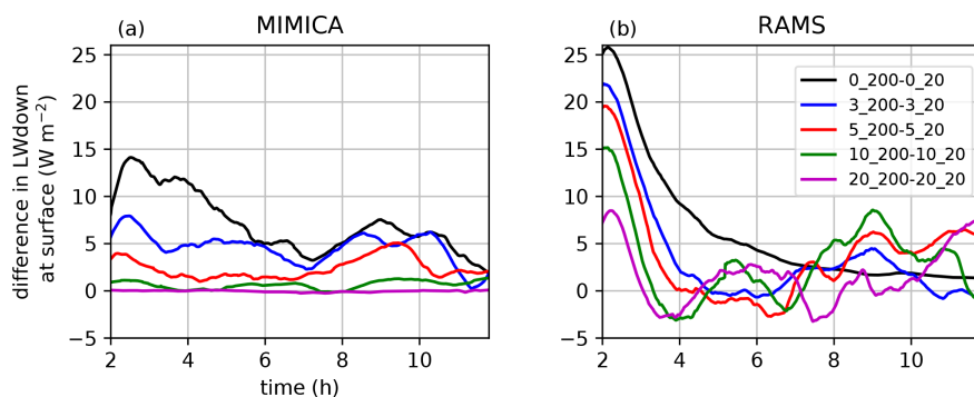
Figure 10. Difference in downward longwave (LWdown) radiation at the surface for simulation pairs with the same accumulation mode concentration (i.e. AC_x\_AK200-AC_x\_AK20 ) shown for (a) MIMICA and (b) RAMS. The first 2 h of simulations, considered as the spin-up period, are excluded. A Student's t test with a 95 % confidence level shows that the (time mean) differences are statistically significantly different for each pair of simulations, except for the pair AC20\_AK200 and AC20\_AK20 in MIMICA. For figure clarity, the plot titles have been abbreviated; the first number refers to the accumulation mode and the second to the Aitken mode concentration in cubic centimetres, i.e. 0_20 refers to AC0\_AK20 .
