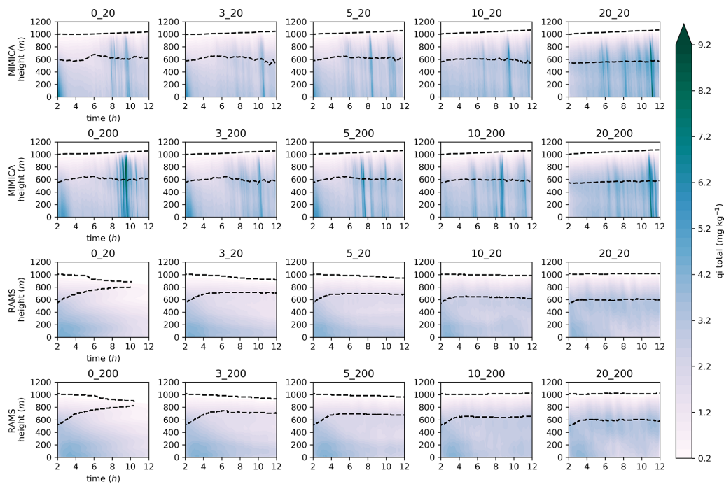
Figure A5. Total ice mixing ratio ( q_i total) for the MIMICA and RAMS simulation sets. The first 2 h of simulations, considered as the spin-up period, are excluded. For figure clarity, the plot titles have been abbreviated; the first number refers to the accumulation mode and the second to the Aitken mode concentration in cubic centimetres, i.e. 0_20 refers to AC0_AK20. Black dashed lines represent the cloud top and cloud base heights.
