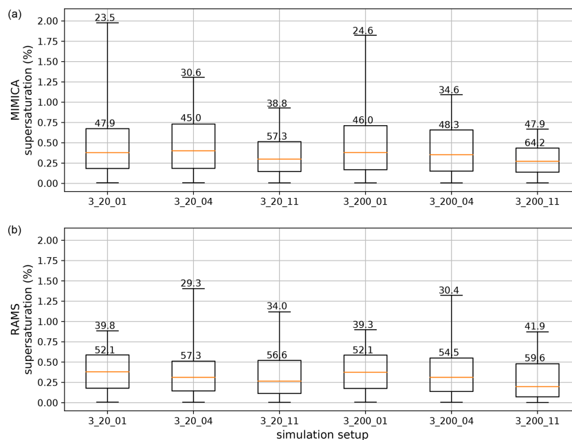
Figure 15. Supersaturation statistics shown for the simulations AC3_AK20 and AC3_AK200 initialized with different \kappa values, which are 0.1, 0.4 and 1.1, simulated by MIMICA and RAMS. The statistics are calculated for a 20 min period around 6 h of simulation for all grid boxes with relative humidity > 100 %. Lower and upper whiskers correspond to 1st and 99th percentiles, respectively. The numbers written in the figure are critical dry diameters that correspond to supersaturation 75th percentiles (upper limit of the box) and 99th percentiles. For figure clarity, the plot titles have been abbreviated; the first number refers to the accumulation mode and the second to the Aitken mode concentration in cubic centimetres, i.e. 3_20_01 refers to AC3_AK20 initialized with a \kappa value of 0.1.
