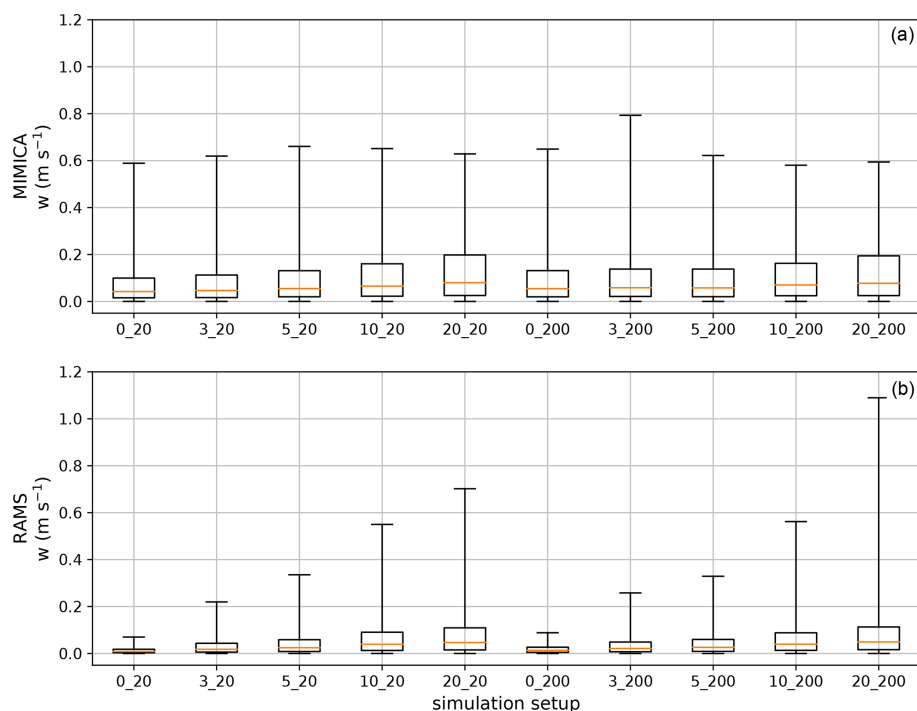
Figure A11. Updraft ( w ) statistics simulated by MIMICA and RAMS. Lower and upper whiskers correspond to first and 99th percentiles, respectively. For figure clarity, the plot titles have been abbreviated; the first number refers to the accumulation mode and the second to the Aitken mode concentration in cubic centimetres, i.e. 0_20 refers to AC0_AK20.
