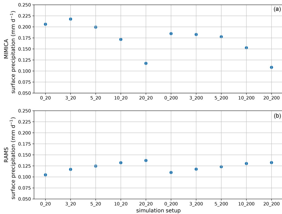
Figure A7. Time mean surface precipitation simulated by MIMICA and RAMS. For figure clarity, the plot titles have been abbreviated; the first number refers to the accumulation mode and the second to the Aitken mode concentration in cubic centimetres, i.e. 0_20 refers to AC0_AK20.
