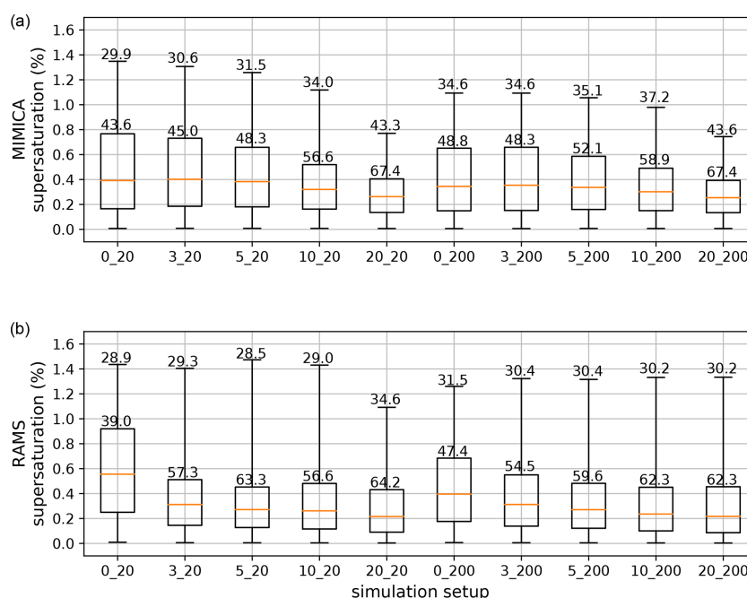
Figure 14. Supersaturation statistics shown for a set of cases initialized with a \kappa value of 0.4, simulated by MIMICA and RAMS. The statistics are calculated for a 20 min period around 6 h of simulation for all grid boxes with relative humidity > 100\% . Lower and upper whiskers correspond to first and 99th percentiles, respectively. The numbers written in the figure are critical dry diameters that correspond to supersaturation 75th percentiles (upper limit of the box) and 99th percentiles. For figure clarity, the plot titles have been abbreviated; the first number refers to the accumulation mode and the second to the Aitken mode concentration in cubic centimetres, i.e. 0_20 refers to AC0_AK20.
