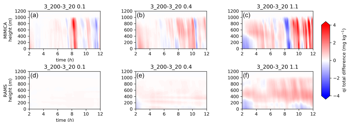
Figure A10. Differences in total ice mixing ratio ( qi total) for simulation pairs with the same accumulation mode concentration and the same \kappa value of the Aitken mode particles equal to 0.1 (a, d), 0.4 (b, e) and 1.1 (c, f) shown for MIMICA and RAMS. The first 2 h of simulations, considered as the spin-up period, are excluded. A Student's t test with a 95 % confidence level shows that the (time mean) differences are statistically significantly different for each pair of simulations. For figure clarity, the plot titles have been abbreviated; the first number refers to the accumulation mode and the second to the Aitken mode concentration in cubic centimetres, i.e. 3_20 refers to AC3_AK20.
