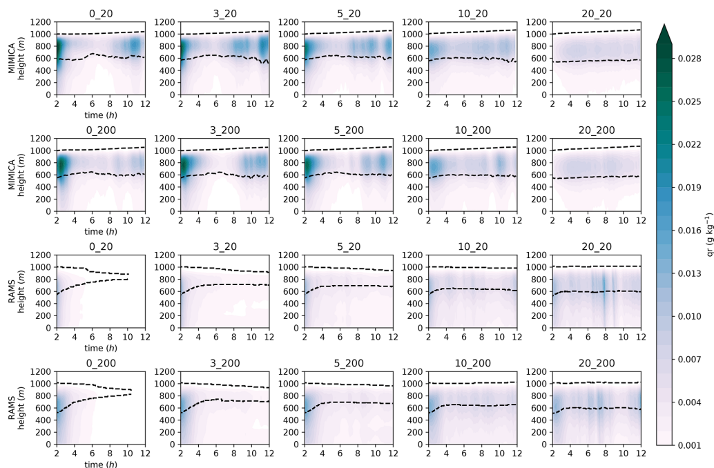
Figure A4. Rain mixing ratio ( q_r ) for the MIMICA and RAMS simulation sets. The first 2 h of simulations, considered as the spin-up period, are excluded. For figure clarity, the plot titles have been abbreviated; the first number refers to the accumulation mode and the second to the Aitken mode concentration in cubic centimetres, i.e. 0_20 refers to AC0_AK20. Black dashed lines represent the cloud top and cloud base heights.
