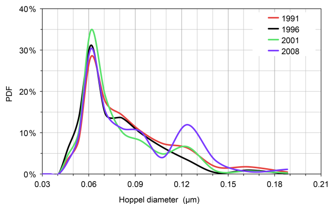
Figure 17. Probability density function (PDF) of the Hoppel diameter shown for four different expeditions in the high Arctic, in the summers of 1991, 1996, 2001 and 2008. Further details on the quality and data processing of the aerosol size resolved measurements are available in Heintzenberg and Leck (2012).
