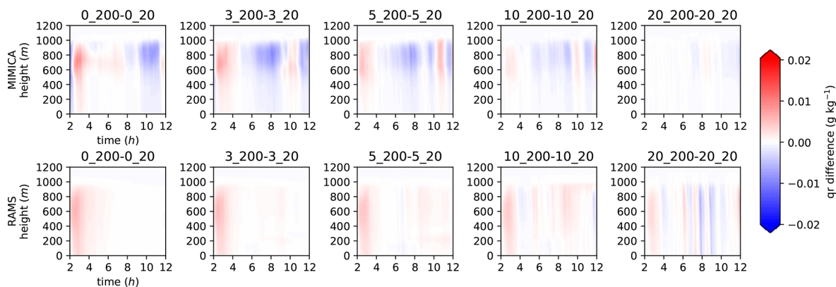
Figure 8. Differences in rain mixing ratio ( q_r ) for simulation pairs with the same accumulation mode concentration (i.e. AC_x\_AK200-AC_x\_AK20 ) shown for MIMICA and RAMS. The first 2 h of simulations, considered as the spin-up period, are excluded. A Student's t test with a 95 % confidence level shows that the (time mean) differences are statistically significantly different for each pair of simulations, except for the pair AC20\_AK200 and AC20\_AK20 in MIMICA. For figure clarity, the plot titles have been abbreviated; the first number refers to the accumulation mode and the second to the Aitken mode concentration in cubic centimetres, i.e. 0\_20 refers to AC0\_AK20 .
