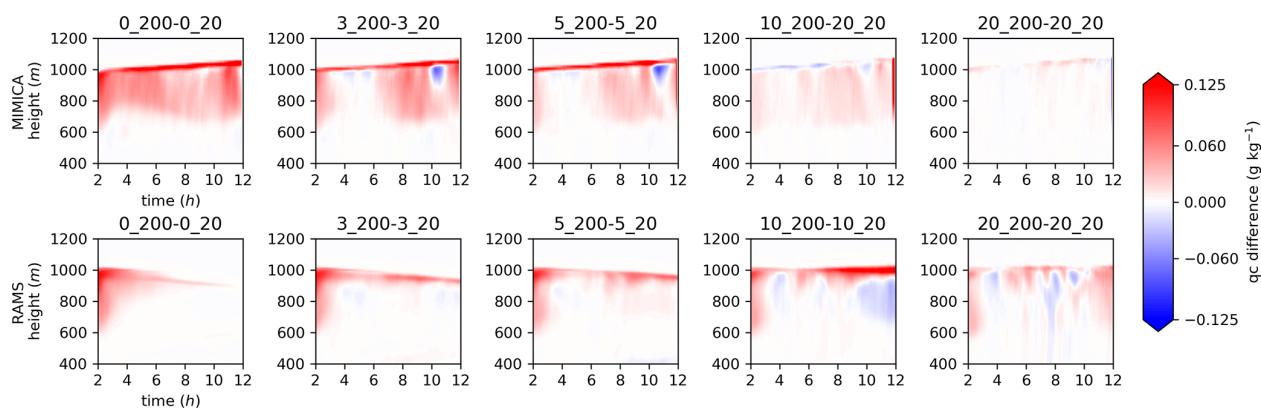
Figure 7. Differences in cloud droplet mixing ratio ( q_c ) for simulation pairs with the same accumulation mode concentration (i.e. AC_x\_AK200-AC_x\_AK20 ) shown for MIMICA and RAMS. The first 2 h of simulations, considered as the spin-up period, are excluded. A Student's t test with a 95 % confidence level shows that the (time mean) differences are statistically significantly different for each pair of simulations, except for the pair AC20\_AK200 and AC20\_AK20 in MIMICA. For figure clarity, the plot titles have been abbreviated; the first number refers to the accumulation mode and the second to the Aitken mode concentration in cubic centimetres, i.e. 0\_20 refers to AC0\_AK20 .
