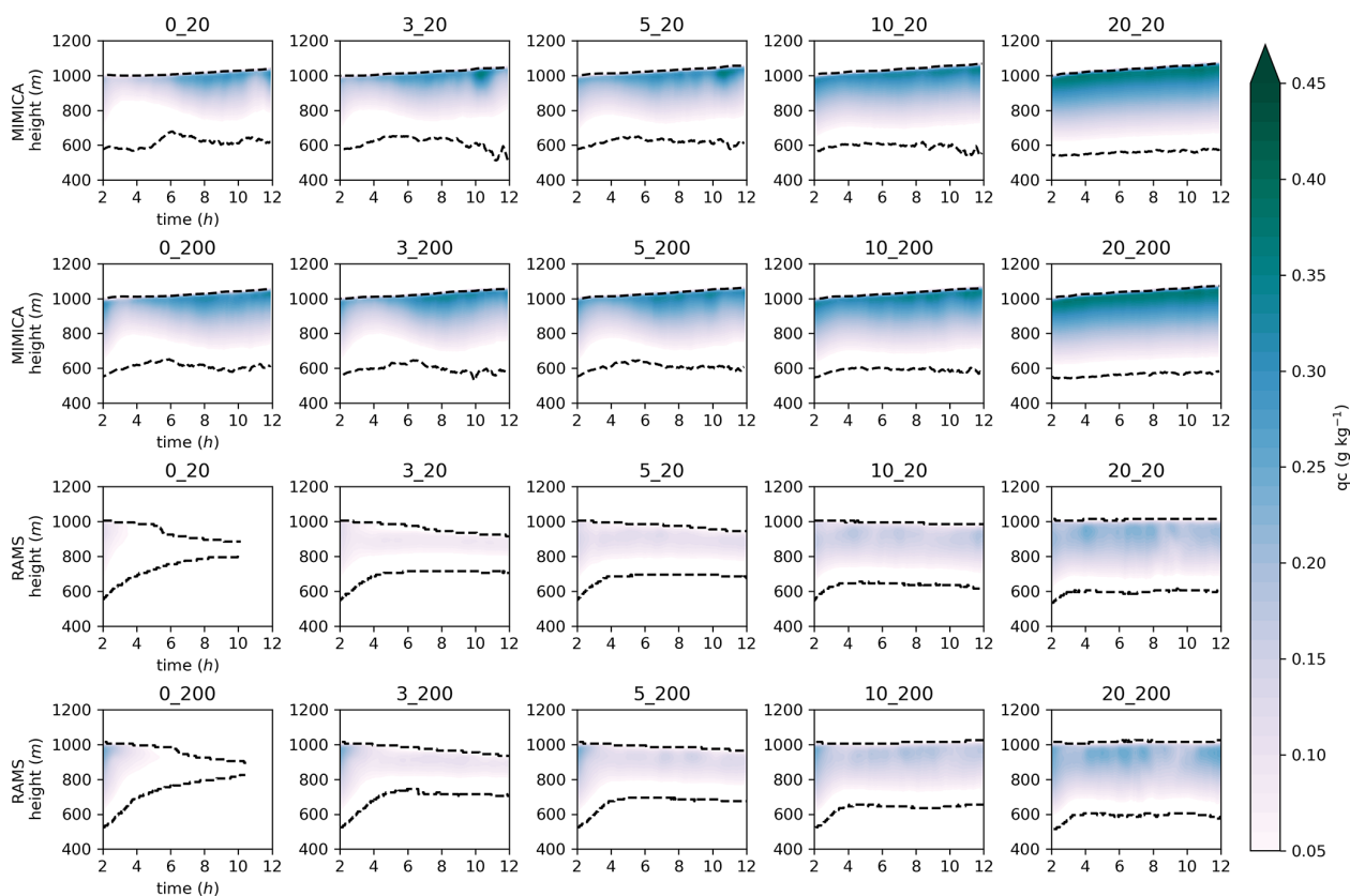
Figure 5. Cloud droplet mixing ratio ( q_c ) for the MIMICA and RAMS simulation sets. The first 2 h of simulations, considered as the spin-up period, are excluded. For figure clarity, the plot titles have been abbreviated; the first number refers to the accumulation mode and the second to the Aitken mode concentration in cubic centimetres, i.e. 0_20 refers to AC0_AK20. Black dashed lines represent the cloud top and cloud base heights.
