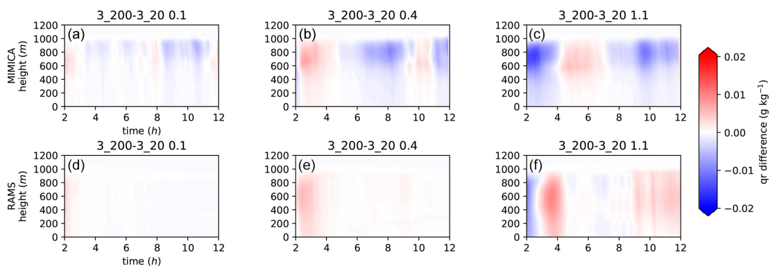
Figure A9. Differences in rain mixing ratio ( qr ) for simulation pairs with the same accumulation mode concentration and the same \kappa value of the Aitken mode particles equal to 0.1 (a, d), 0.4 (b, e) and 1.1 (c, f) shown for MIMICA and RAMS. The first 2 h of simulations, considered as the spin-up period, are excluded. A Student's t test with a 95 % confidence level shows that the (time mean) differences are statistically significantly different for each pair of simulations. For figure clarity, the plot titles have been abbreviated; the first number refers to the accumulation mode and the second to the Aitken mode concentration in cubic centimetres, i.e. 3_20 refers to AC3_AK20.
