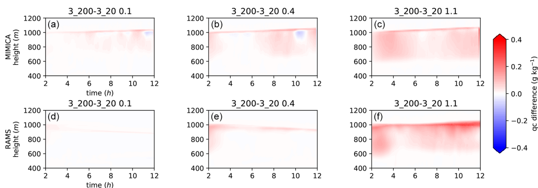
Figure 13. Differences in cloud droplet mixing ratio ( q_c ) for simulation pairs with the same accumulation mode concentration and the same \kappa value of the Aitken mode particles equal to 0.1 (a, d), 0.4 (b, e) and 1.1 (c, f) shown for MIMICA and RAMS. The first 2 h of simulations, considered as the spin-up period, are excluded. A Student's t test with a 95 % confidence level shows that the (time mean) differences are statistically significantly different for each pair of simulations. For figure clarity, the plot titles have been abbreviated; the first number refers to the accumulation mode and the second to the Aitken mode concentration in cubic centimetres, i.e. 0_20 refers to AC0_AK20.
