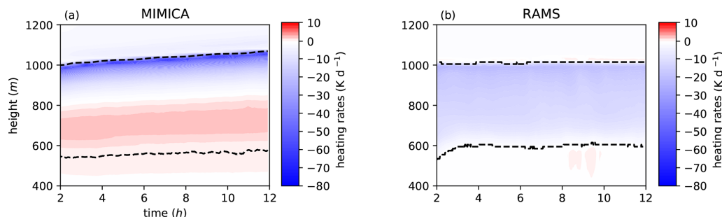
Figure 6. Radiative heating rates in the baseline simulation (AC20_AK20), simulated by (a) MIMICA and (b) RAMS. The first 2 h of simulations, considered as the spin-up period, are excluded. Black dashed lines represent the cloud top and cloud base heights.
