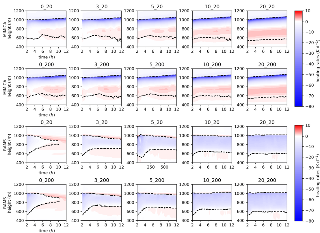
Figure A2. Radiative heating rates for the MIMICA and RAMS simulation sets. The first 2 h of simulations, considered as the spin-up period, are excluded. For figure clarity, the plot titles have been abbreviated; the first number refers to the accumulation mode and the second to the Aitken mode concentration in cubic centimetres, i.e. 0_20 refers to AC0_AK20. Black dashed lines represent the cloud top and cloud base heights.
