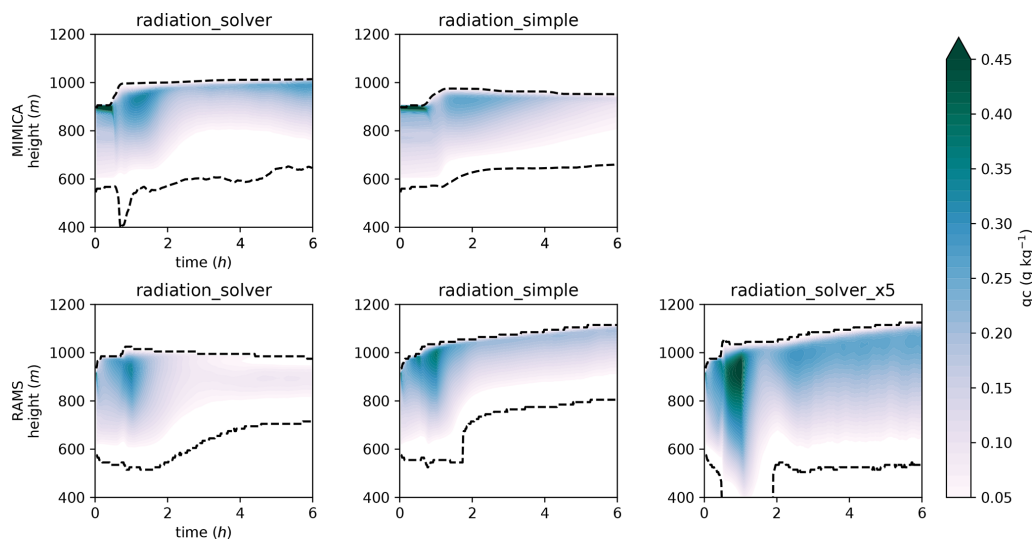
Figure A1. Cloud droplet mixing ratio ( q_c ) shown for a simulation AC3_AK20 initialized with different radiative schemes in MIMICA and RAMS. The title radiation_solver is used for the simulations in which the models are initialized with their default radiation solvers (Fu and Liou, 1993, in MIMICA and Harrington, 1997, in RAMS). The title radiation_simple is used for the simulations where the radiative fluxes are calculated as functions of LWP only (Stevens et al., 2005, in MIMICA and Chen and Cotton, 1983, in RAMS). The radiation_solver_x5 simulated by RAMS shows the q_c obtained with the default radiation solver but with a 5\times higher cooling rate enforced at cloud top. The simulations are run for 6 h. Black dashed lines represent the cloud top and cloud base heights.
