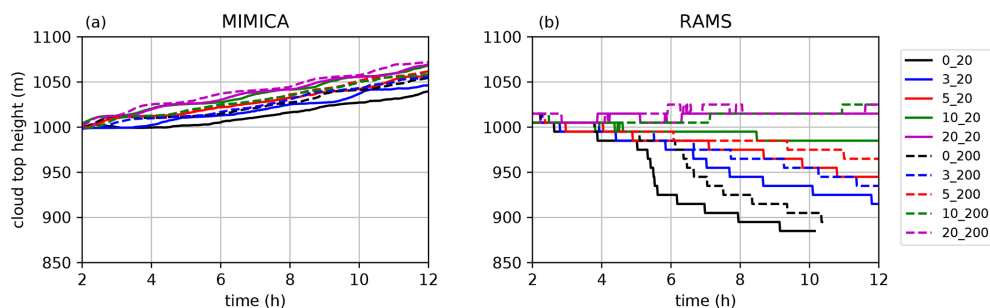
Figure A3. Cloud top heights in (a) MIMICA and (b) RAMS. The first 2 h of simulations, considered as the spin-up period, are excluded.
