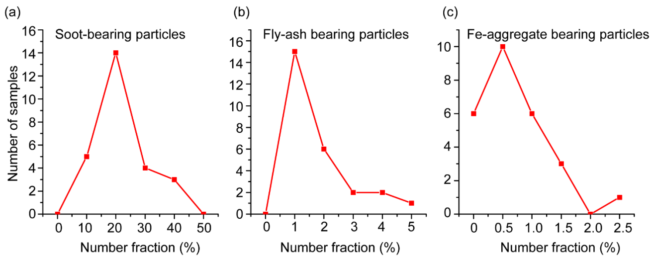
65 Figure S9. Histogram of the number fractions of the particles containing inclusions. (a) Soot-bearing particle number fractions. (b) Fly-ash bearing particle number fractions. (c) Fe-aggregate-bearing particle number fractions. The average values of these number fractions are 17%, 1.4%, and 0.5%, respectively.
