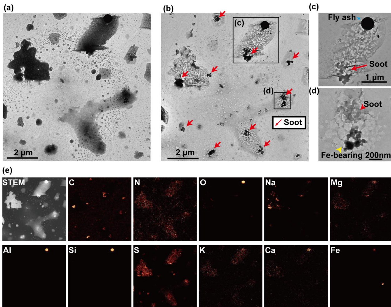
Figure S8. TEM and elemental mapping images of the sulfate particles containing inclusions. (a) TEM image before the mapping analysis and (b) after the mapping analysis. Electron-beam exposure removed sulfate, and the inclusions became more apparent. (c) A particle in the image (b) with fly-ash and soot inclusions. (d) A particle with Fe-aggregate and soot inclusions. (e) Elemental mapping images of the TEM areas of the detected elements. The C distributions in the mapping image correspond to the soot particles. The fly-ash particle in (c) includes O, Al, and Si as its main components. Fe is apparent in the Fe-aggregate particle in (d). The sample was collected from 14:40-14:59, 31 March 2018.
