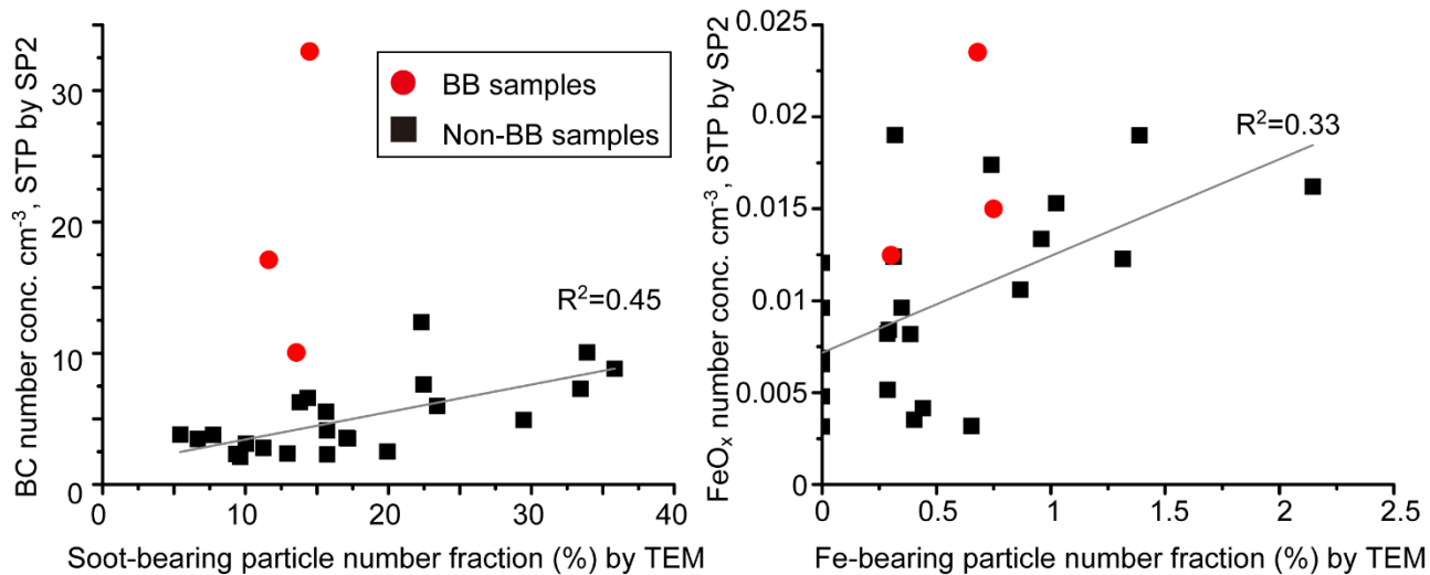
Figure S12. Relations between TEM and SP2 measurement for Soot/BC and Fe-bearing particles/FeO x . Left: Soot-bearing particle number fraction by TEM vs. BC number concentrations by SP2. Right: Fe-bearing particle number fraction vs. FeO x number concentration by SP2. Red plots indicate BB samples. The correlations were calculated for non-BB samples.
