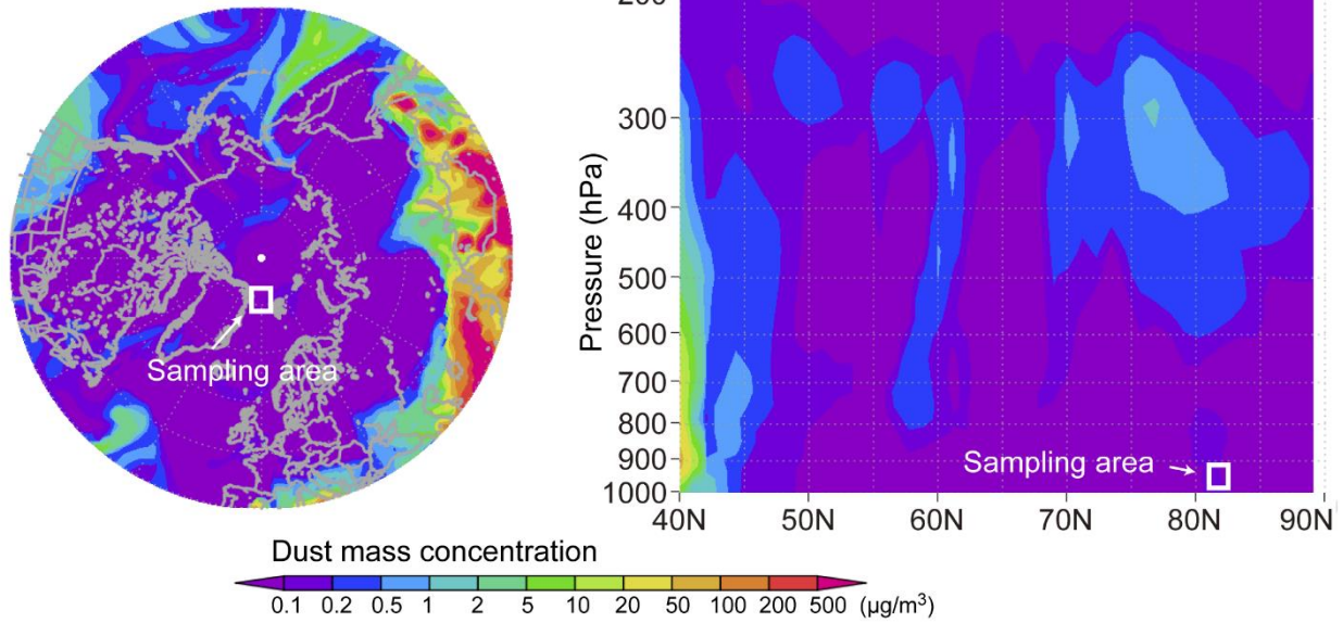
50 Figure S7. Example model results of the (a) horizontal and (b) vertical distributions of the mineral-dust mass concentration on 12:00 UTC, 30 March 2018. The mineral-dust number fractions in the TEM analysis were relatively high on that day, but no dust plume was detected in the model. The vertical distribution is shown along the 10° E longitude. The sampling area is shown in the white squares.
