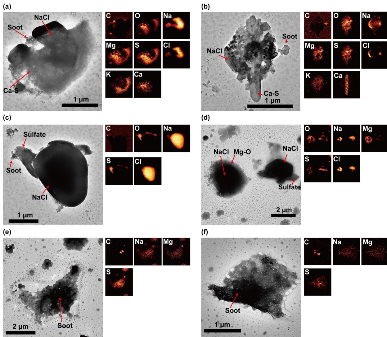
30 Figure S3. TEM and elemental mapping images of the sea-salt particles. The particles in (a), (b), (c), and (d) were collected from 10:00-10:19, 30 March, 2018, and those in (e) and (f) were collected from 14:40-14:59, 31 March. The left TEM image in each panel shows the sea-salt particles mixed with various grains. Elemental mapping images of the TEM areas for the detected elements are shown on the right in each panel. Chlorine was not detected in the particles in (e) and (f) because of Cl replacement 35 with sulfate in the atmosphere.
