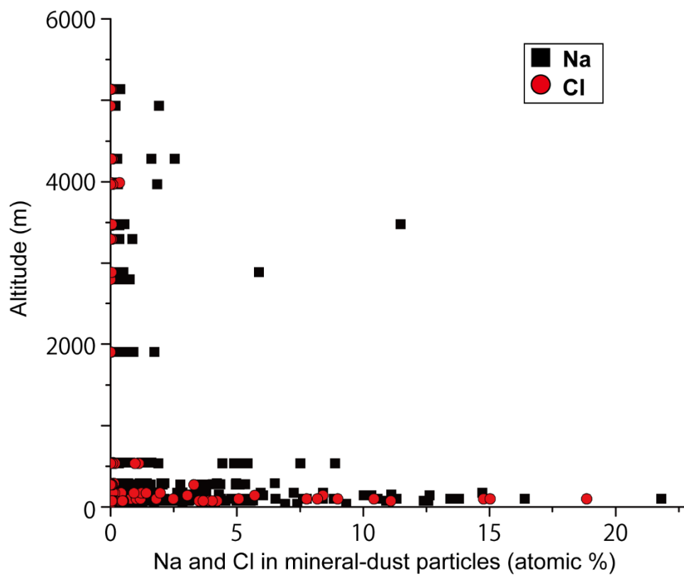
45 Figure S6. Atomic percent of Na (black) and Cl (red) within all mineral-dust particles along with their sampling altitude. The sea-salt fractions within the individual mineral-dust particles are high at a low altitude.
