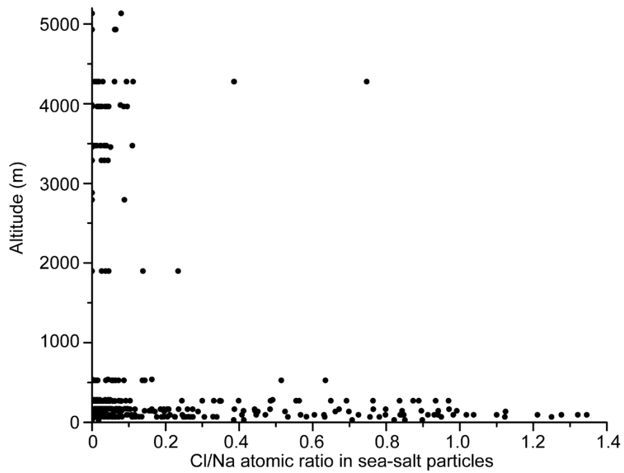
Figure S4. Ratios of Cl to Na in the atomic ratio for all individual sea-salt particles. Chlorine was largely lost in the particles collected above 1000 m.
