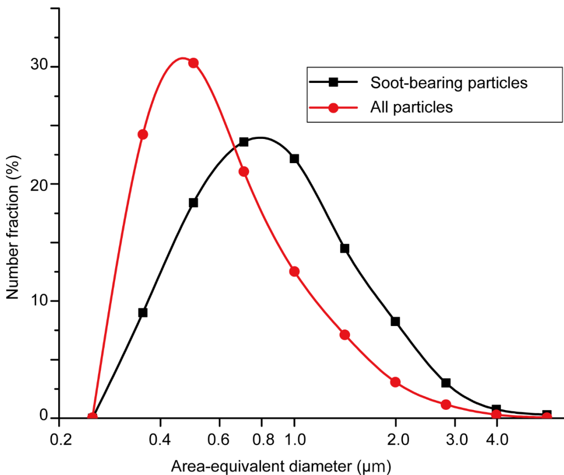
Figure S10. Size distributions of the soot-bearing particles (black line) and all particles (red line). The size bins are shown on a log scale ( < 0.25 , 0.25-0.35 , 0.35-0.5 , 0.5-0.71 , 0.71-1.00 , 1.00-1.41 , 1.41-2.00 , 2.00-2.82 , 2.82-3.98 , and >3.98 \mu\text{m} ). The sizes of the soot-bearing particles reflect those of their host particles. The numbers of all particles and soot-bearing particles are 7844 and 1331, respectively.
