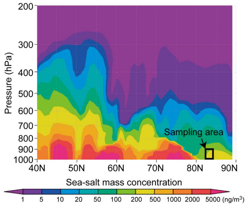
40 Figure S5. Example model result of the vertical distribution of the sea-salt mass concentration on 12:00 UTC, 30 March 2018 at 0° E longitude. The sea-salt number fractions in the TEM analysis were relatively high on that day. The sampling area is shown in a black square.
