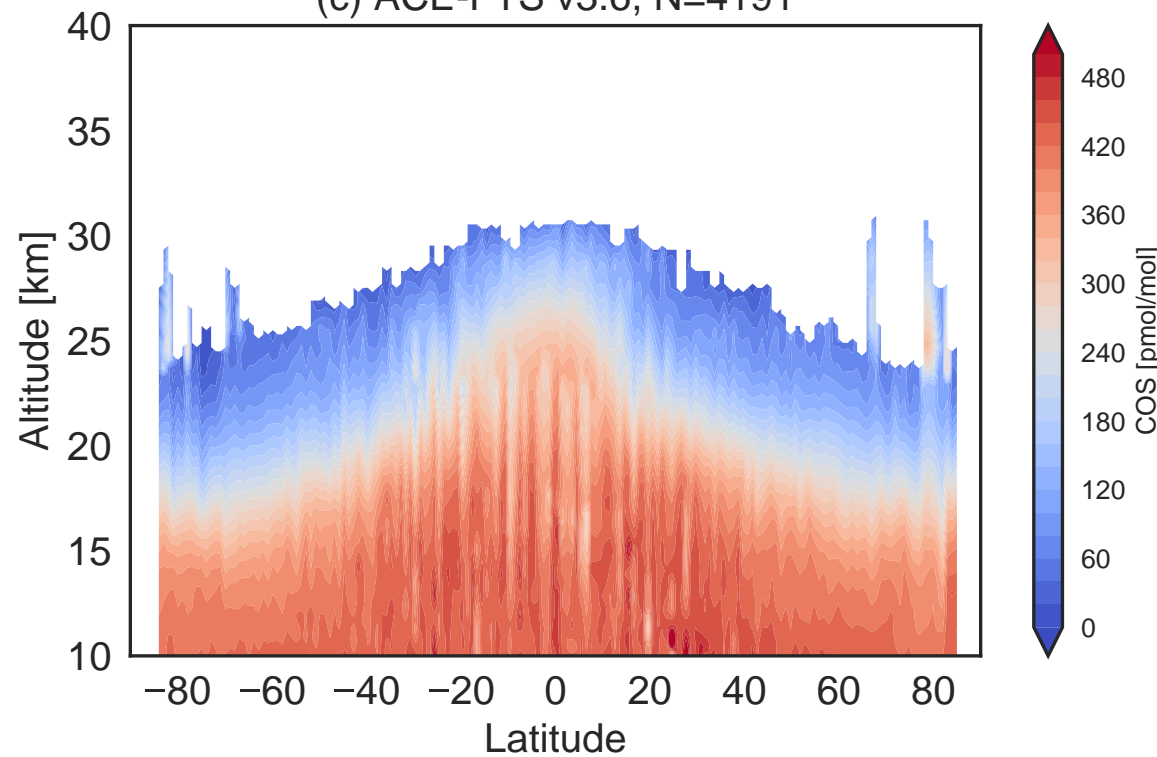
(c) ACE-FTS v3.6, N=4191
