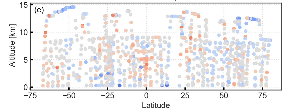
Post-Obs HIPPO optimized
