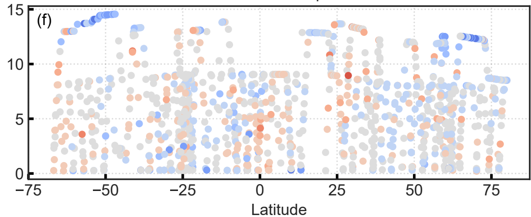
Post-Obs HIPPO optimized
