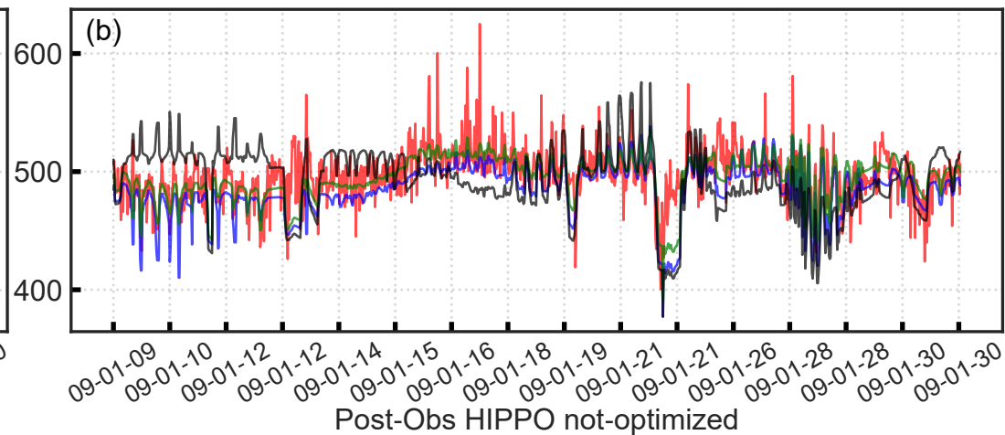
HIPPO campaign-1 S u
