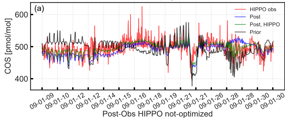
HIPPO campaign-1 S 1
