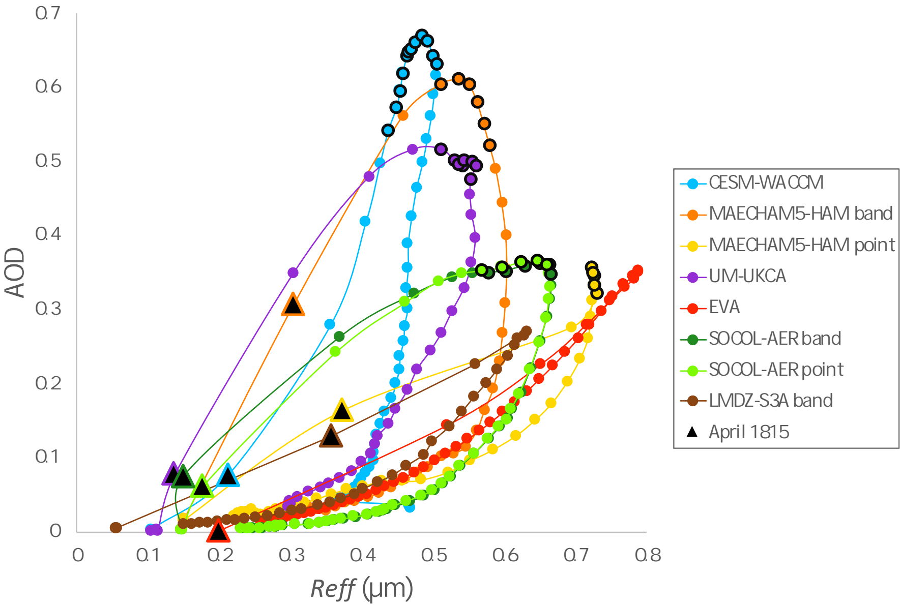
Global Stratospheric Average AOD vs. Reff
