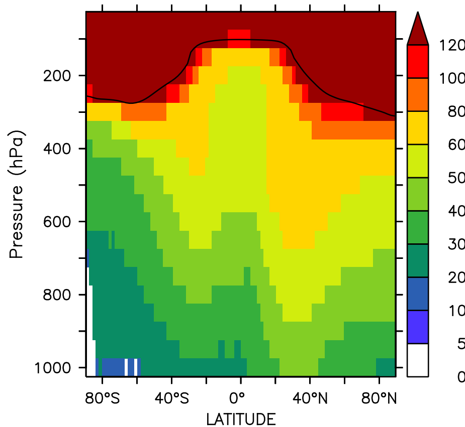
(a) onlyMCM: O3 annual mean ( \times 10^{-9} mol/mol)
