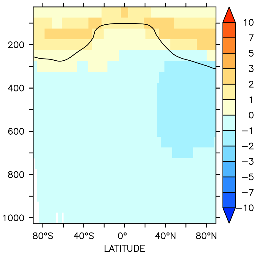
(b) O3 absolute difference ( \times 10^{-9} mol/mol)
