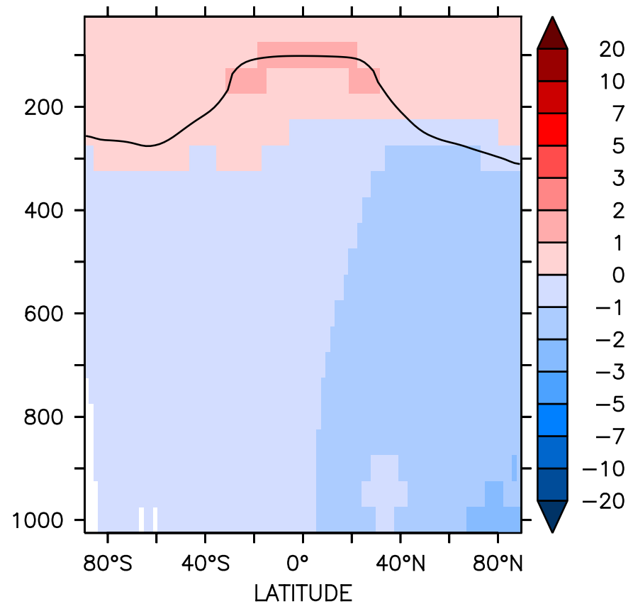
(c) O3 relative difference (%)
