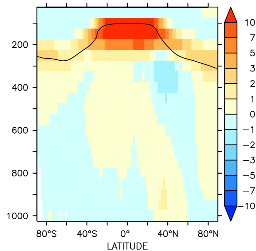
(b) OH absolute difference ( \times 10^{-15} mol/mol)
