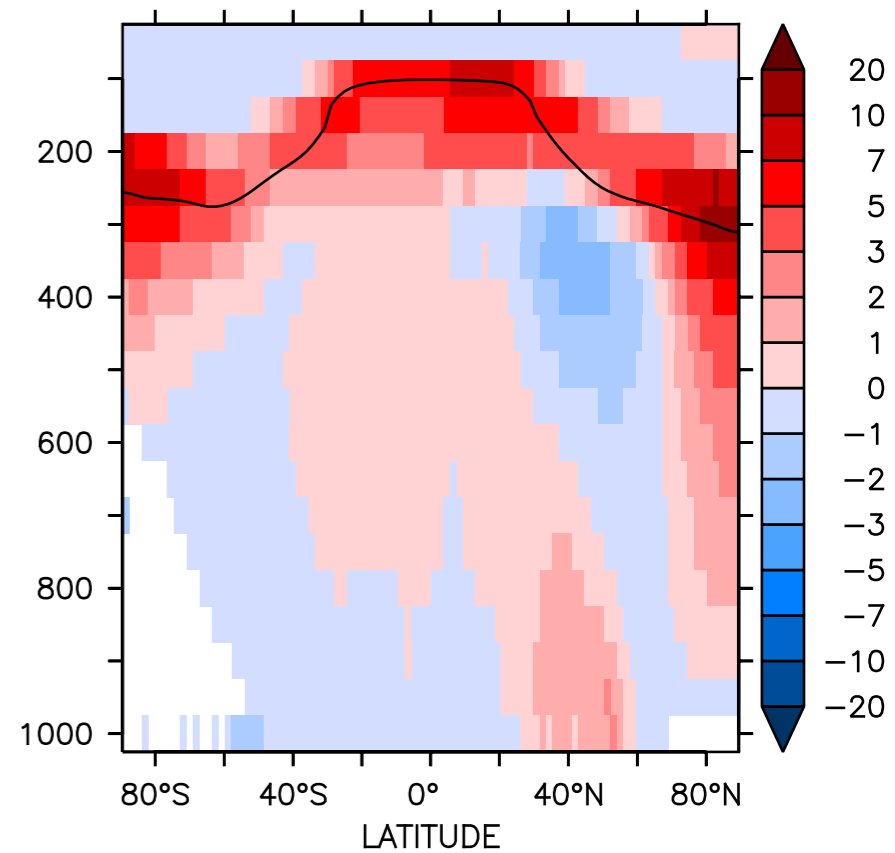
(c) OH relative difference (%)
