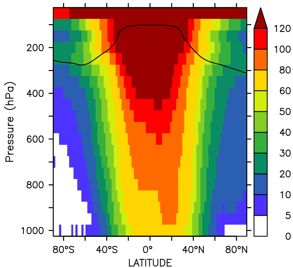
(a) onlyMCM: OH annual mean ( \times 10^{-15} mol/mol)
