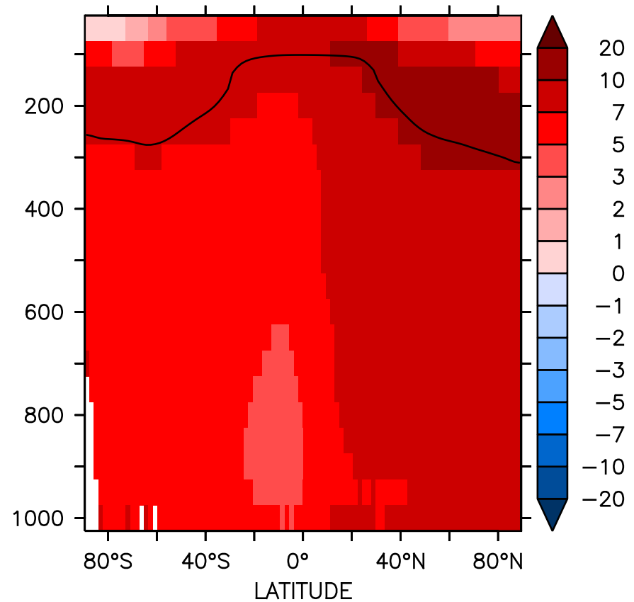
(c) CO relative difference (%)
