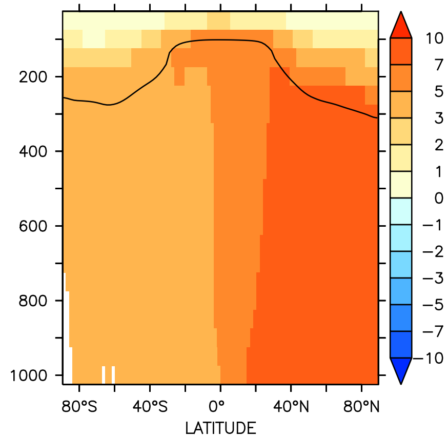
(b) CO absolute difference ( \times 10^{-9} mol/mol)
