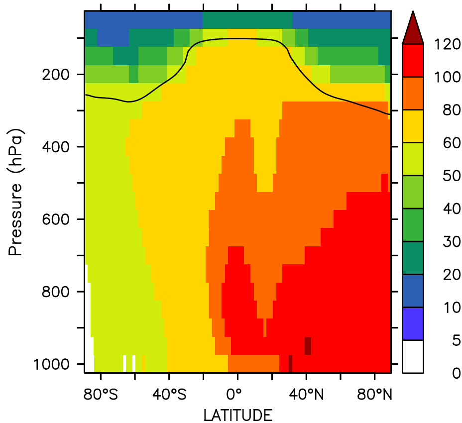
(a) NOAROM: CO annual mean ( \times 10^{-9} mol/mol)
