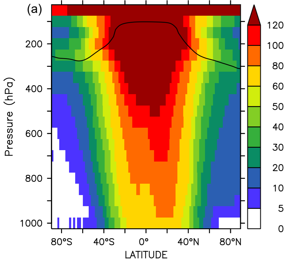
NOAROM: OH annual mean ( \times 10^{-15} mol/mol)
