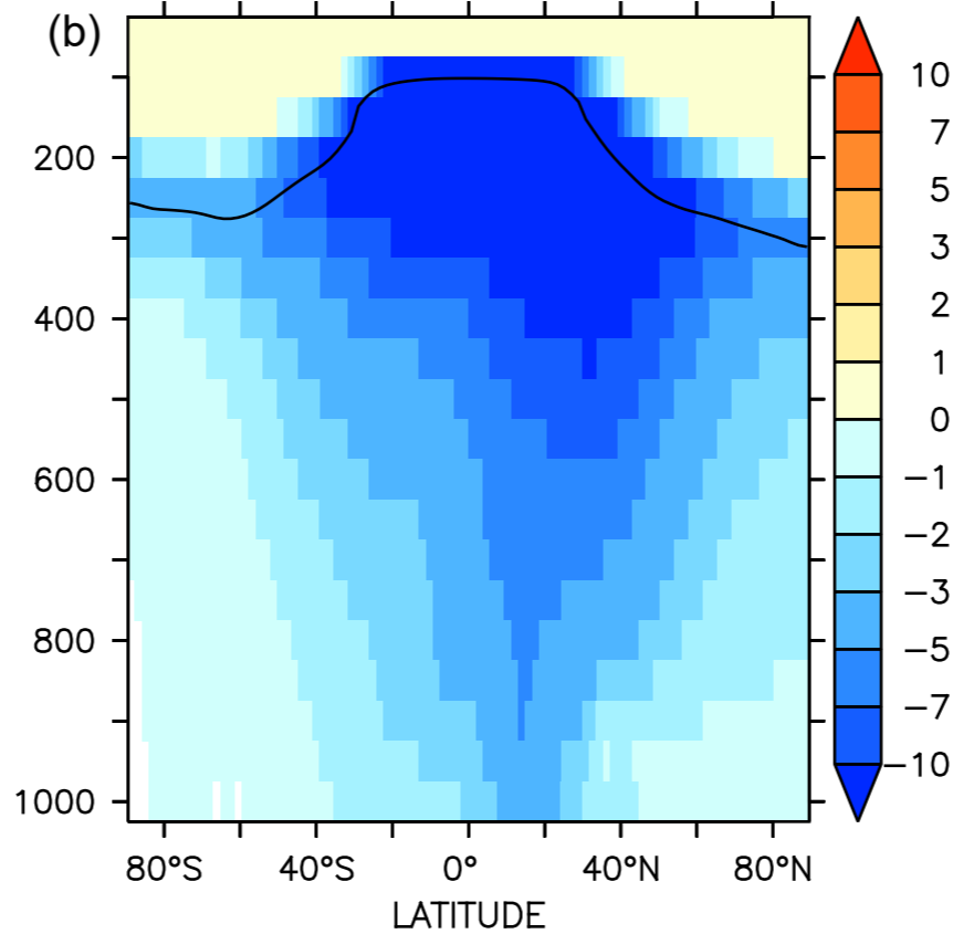
OH absolute difference ( \times 10^{-15} mol/mol)
