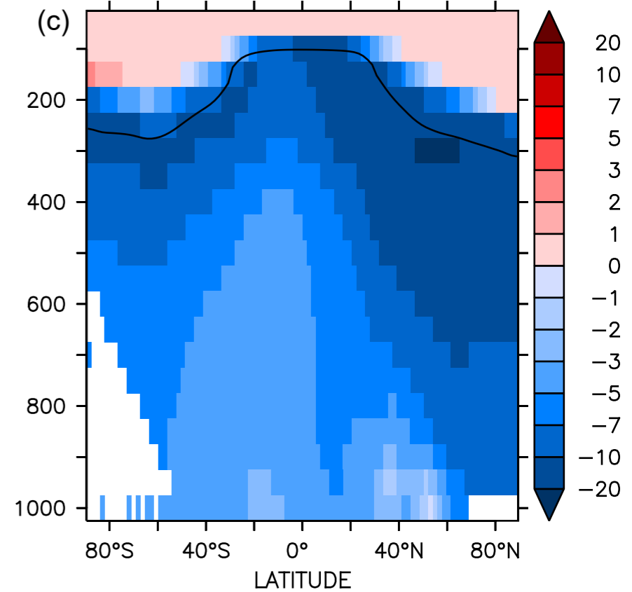
OH relative difference (%)
