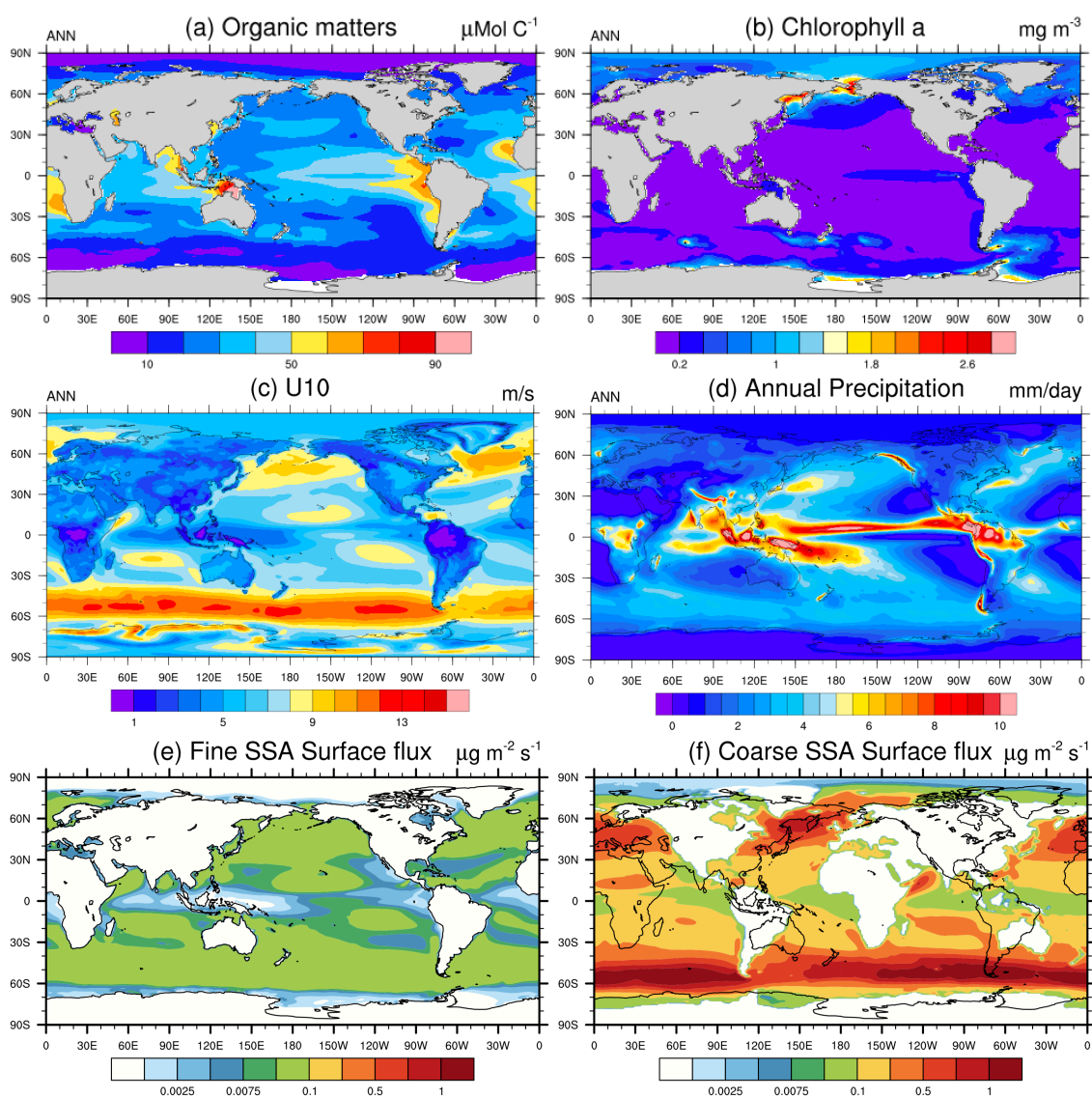
Figure S1. Spatial distributions of (a) ocean organic matter concentration, (b) ocean Chl-a concentration, (c) 10-meter wind speed, (d) annual precipitation, (e) fine mode SSA surface flux, and (f) Coarse mode SSA surface flux.
