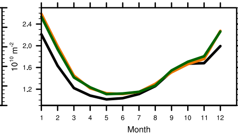
(e) SWCF
