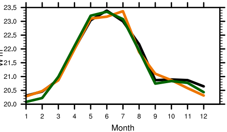
(i) LWCF
