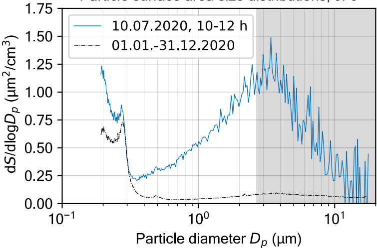
Particle surface area size distributions, JFJ
