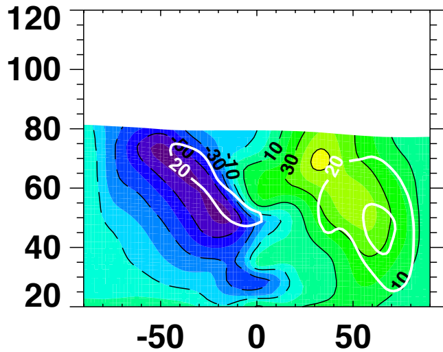
WACCMX+DART
