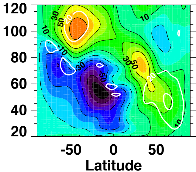
WACCMX+DART
