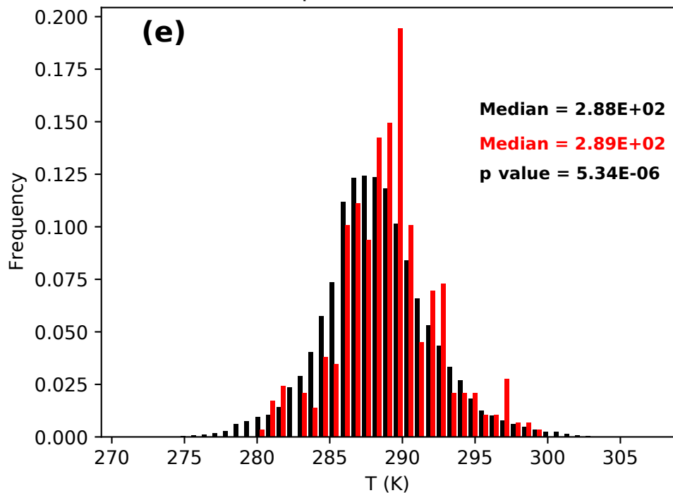
Temperature at 850 hPa
