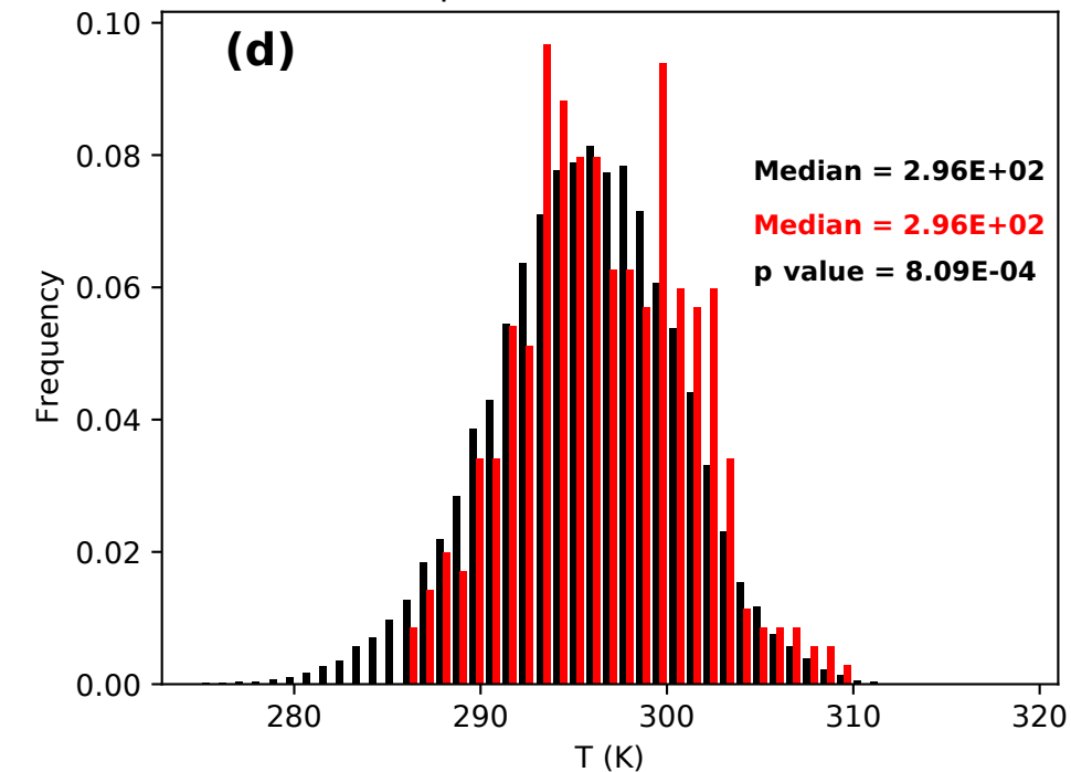
Temperature at 2 m altitude
