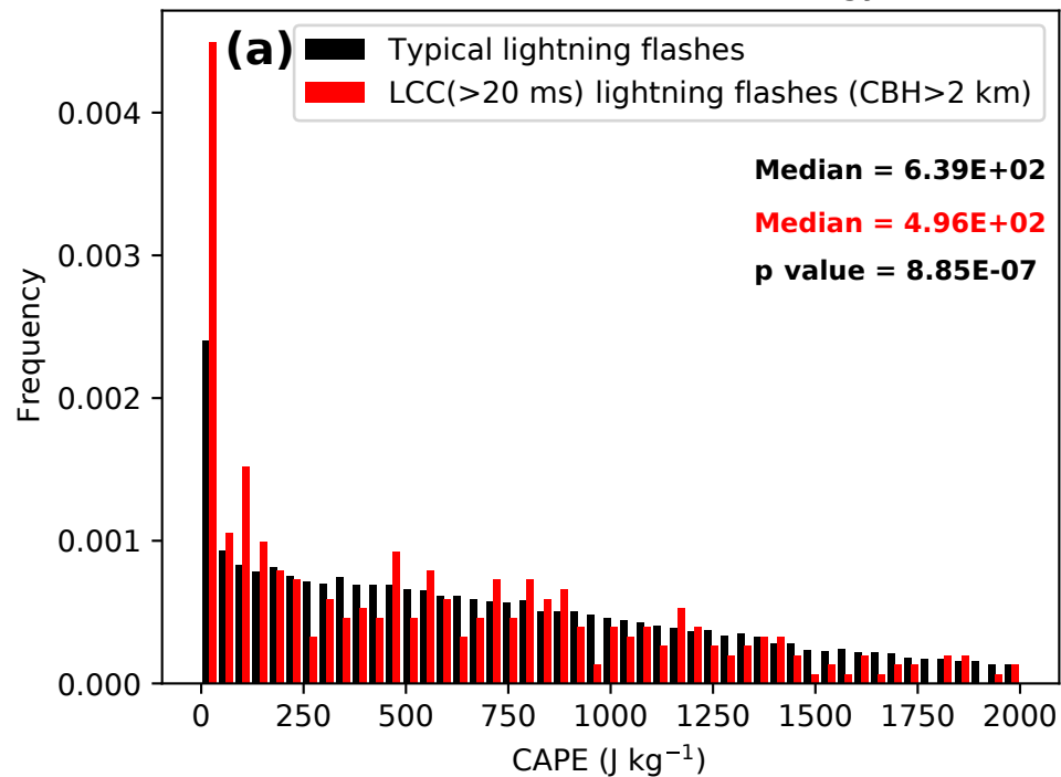
Convective Available Potential Energy (CAPE)
