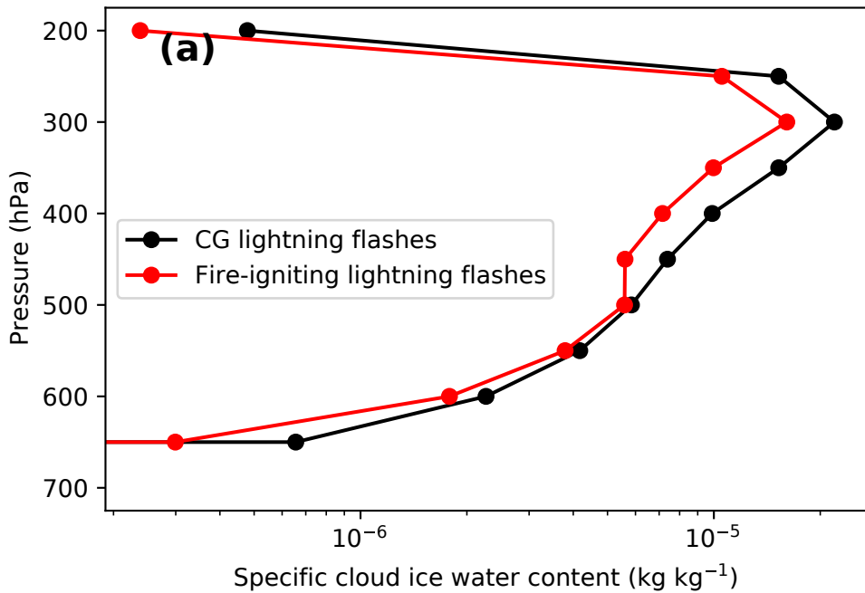
Iberian Peninsula Specific cloud ice water content profile
