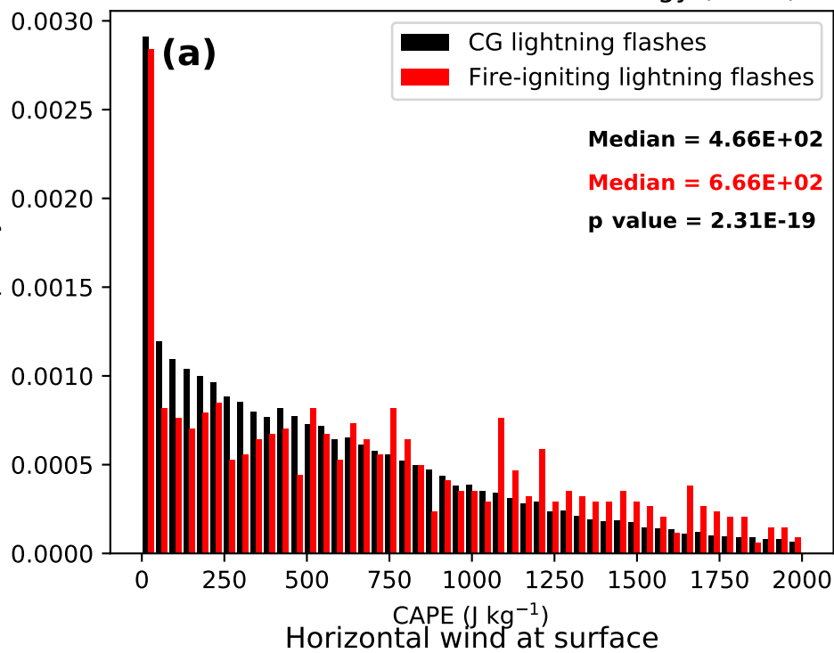
Convective Available Potential Energy (CAPE)
