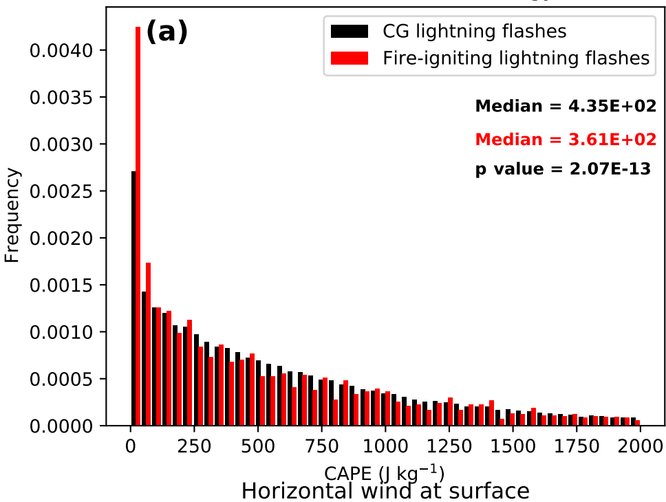
Convective Available Potential Energy (CAPE)
