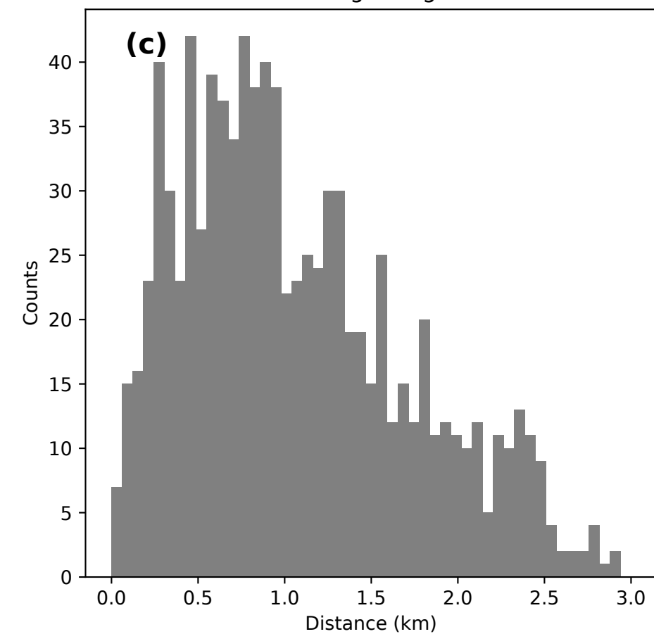
Distance fire-lightning candidate
