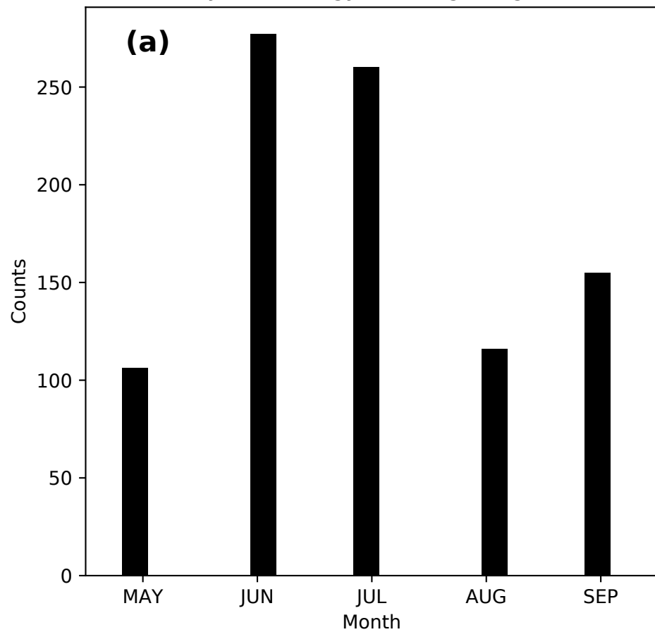
Monthly climatology of fire-igniting flashes
