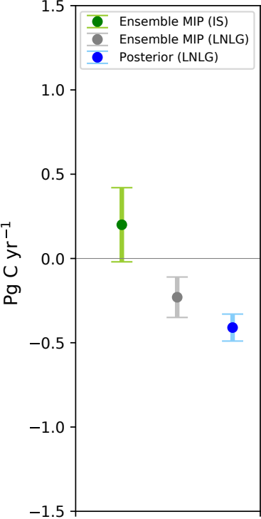
(a) Annual land biosphere CO 2 flux
