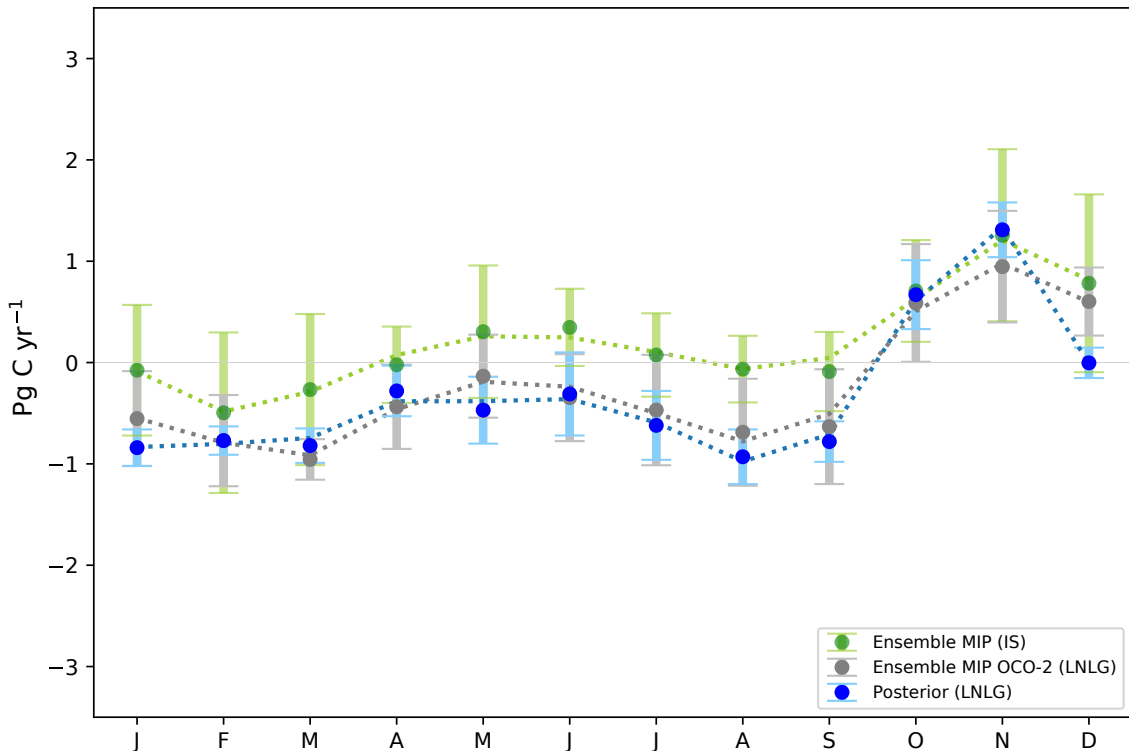
(b) Australian land biosphere CO 2 flux for 2015
