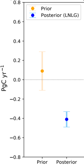
(a) Annual terrestrial CO 2 flux
