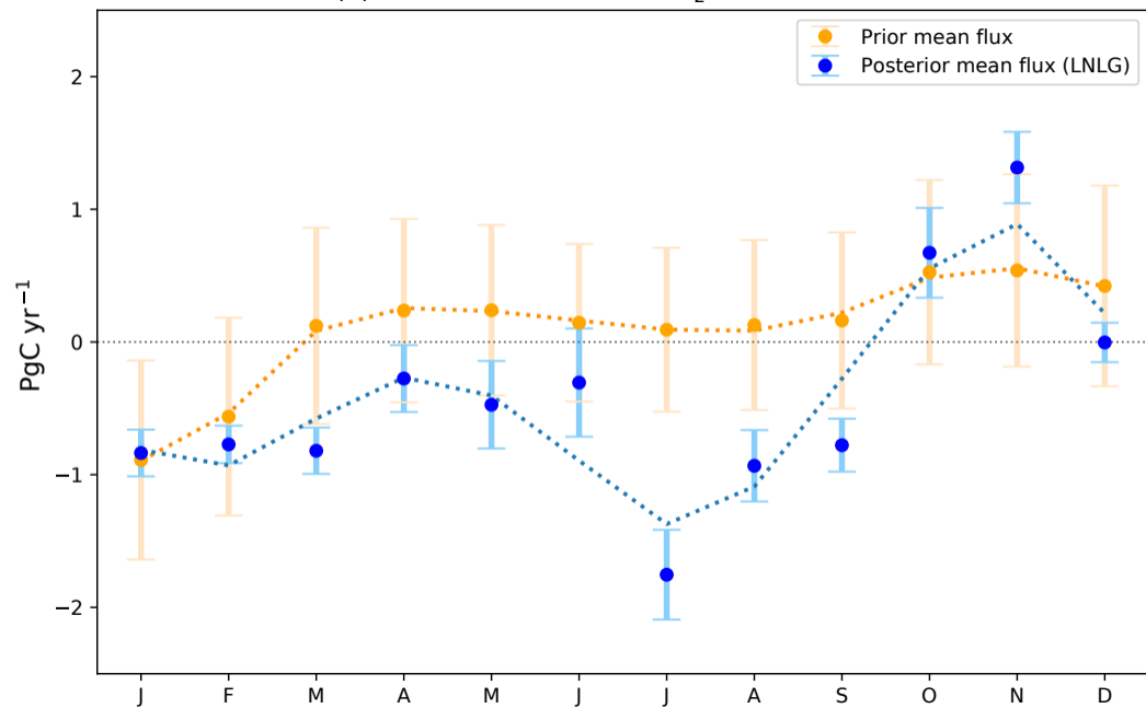
(b) Australian terrestrial CO 2 fluxes for 2015
