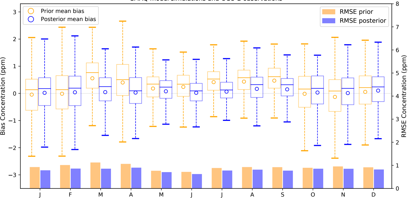
CMAQ model simulations and OCO-2 observations
