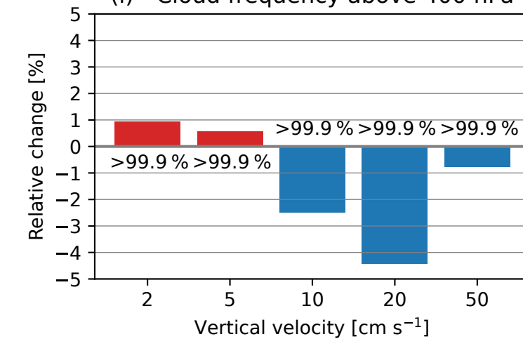
(i) - Cloud frequency above 400 hPa
