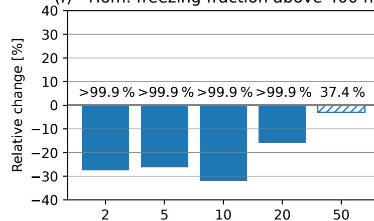
(f) - Hom. freezing fraction above 400 hPa
