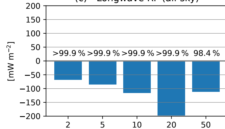
(c) - Longwave RF (all-sky)
