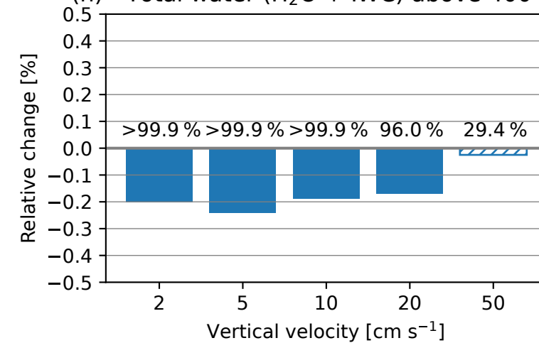
(h) - Total water (H 2 O + IWC) above 400 hPa
