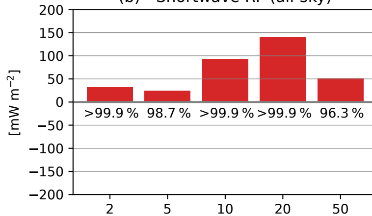
(b) - Shortwave RF (all-sky)
