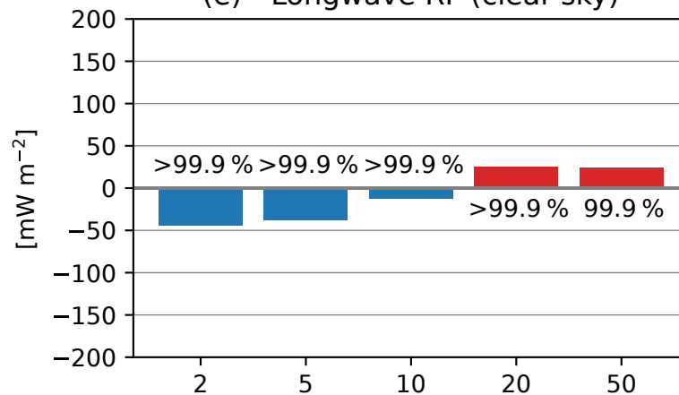
(e) - Longwave RF (clear-sky)
