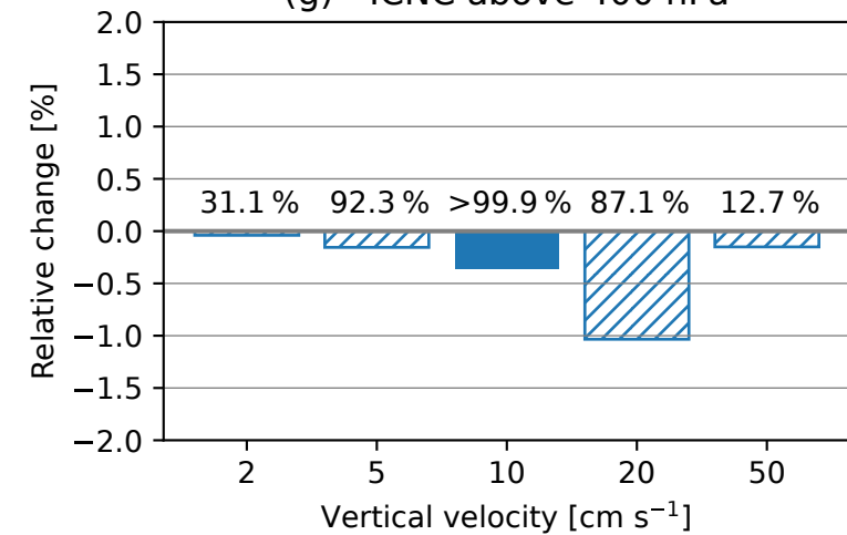
(g) - ICNC above 400 hPa
