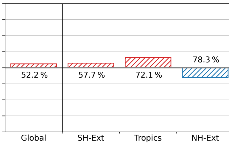
(h) - S_{\text{crit}}=1.3, f_{\text{act}}=0.1\%
