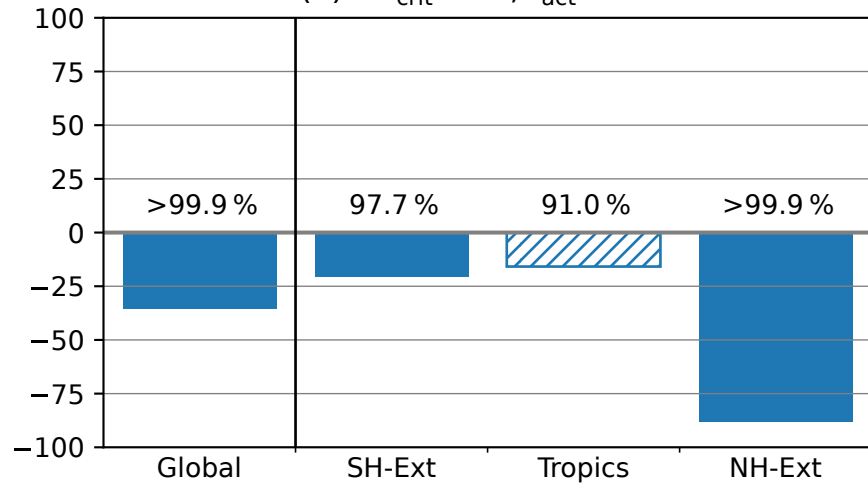
(a) - S_{\text{crit}}=1.2, f_{\text{act}}=10\%
