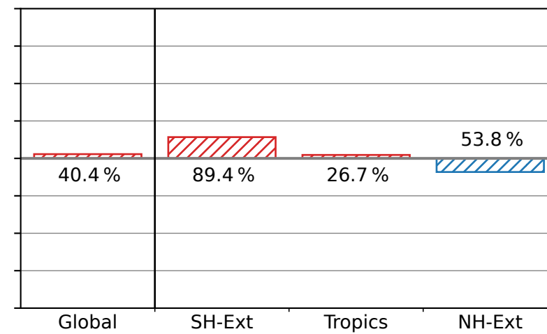
(i) - S_{\text{crit}}=1.4, f_{\text{act}}=0.1\%
