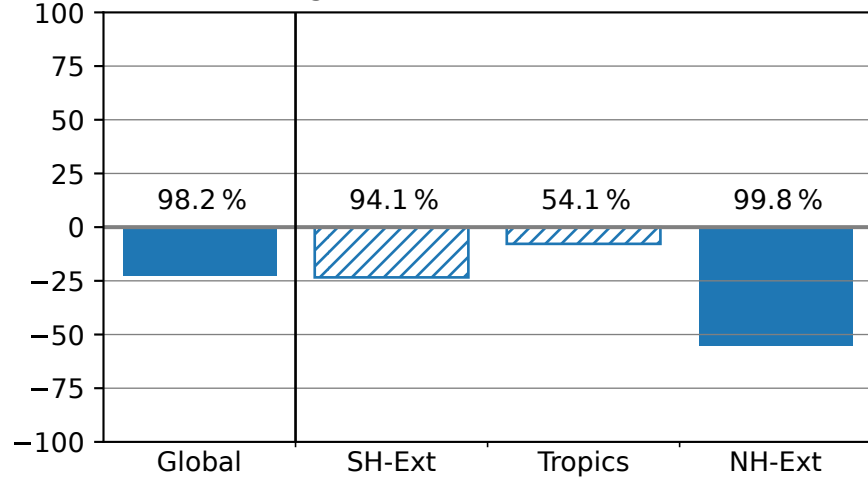
(g) - S_{\text{crit}}=1.2, f_{\text{act}}=0.1\%
