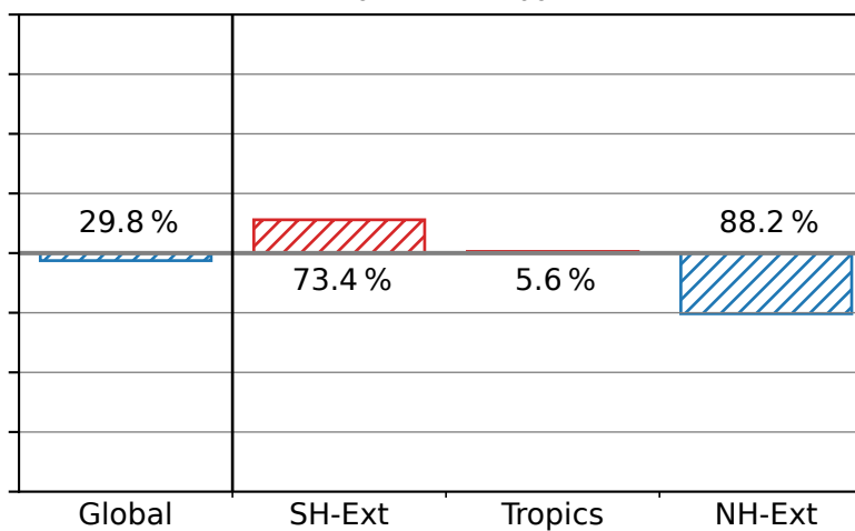
(e) - S_{\text{crit}}=1.3, f_{\text{act}}=1\%
