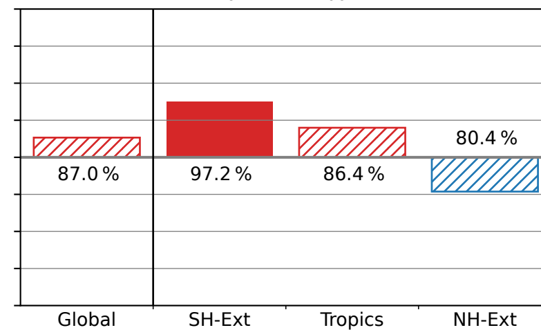
(f) - S_{\text{crit}}=1.4, f_{\text{act}}=1\%
