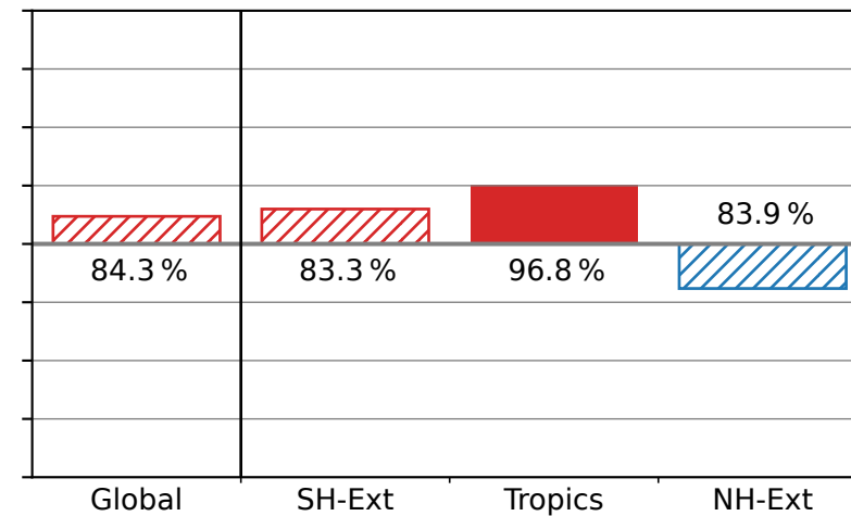
(c) - S_{\text{crit}}=1.4, f_{\text{act}}=10\%
