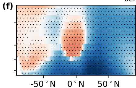
OsloAeroSec-OsloAero def
