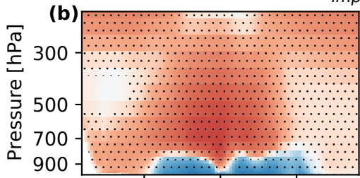
OsloAeroSec-OsloAero def
