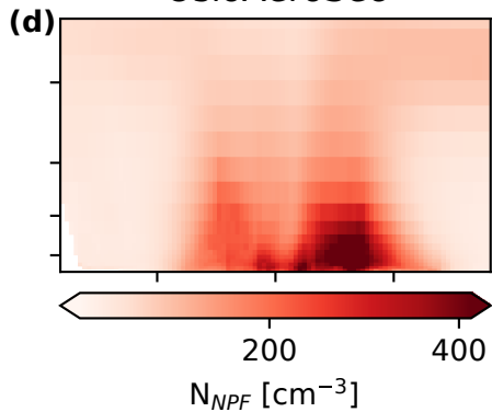
PD OsloAeroSec
