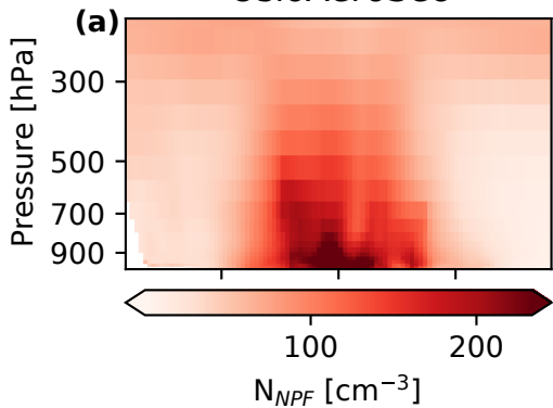
Pre-industrial OsloAeroSec
