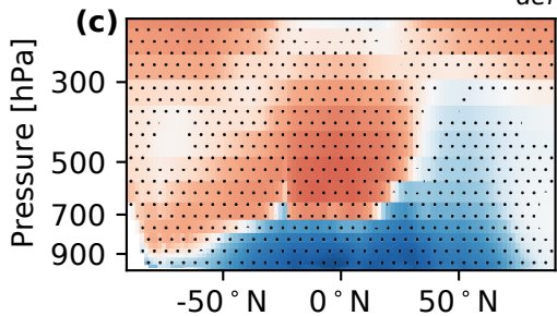
OsloAeroSec-OsloAero def
