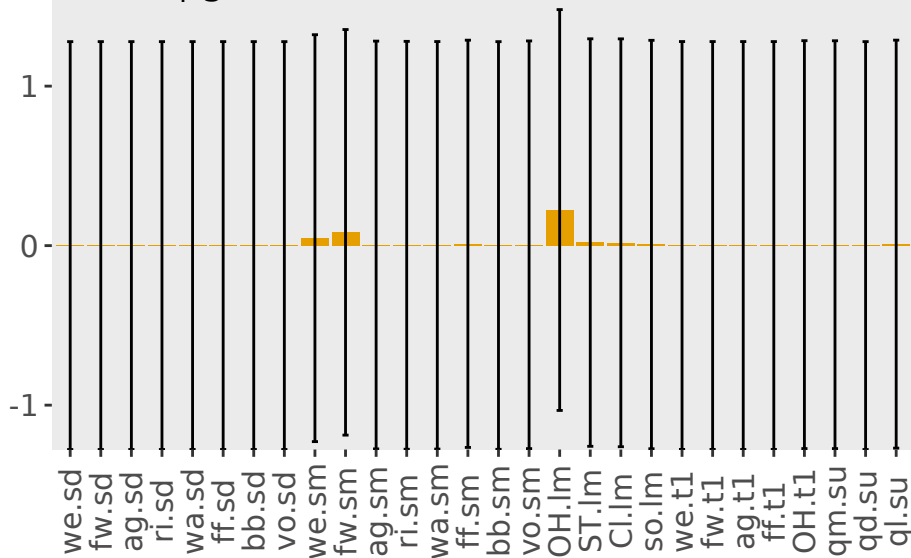
(c) CH 4 inter-hemispheric difference
