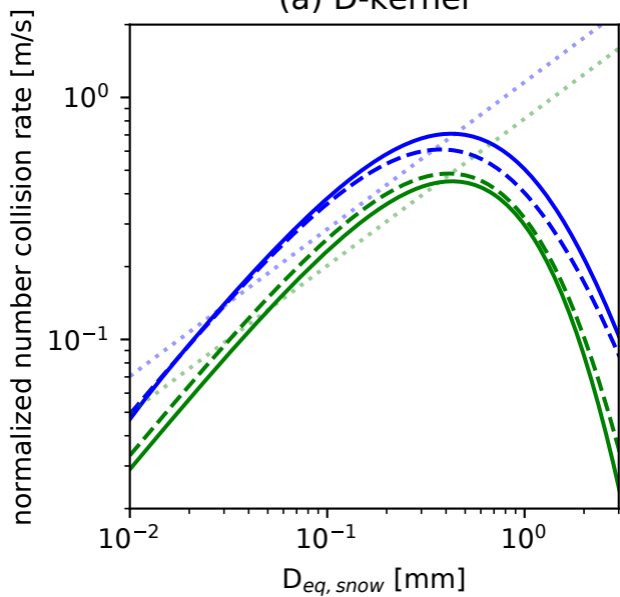
(a) D-kernel
