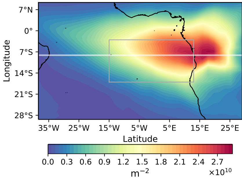
(a) Spatial budget [TM:7.0e+09, CBM:1.5e+10]
