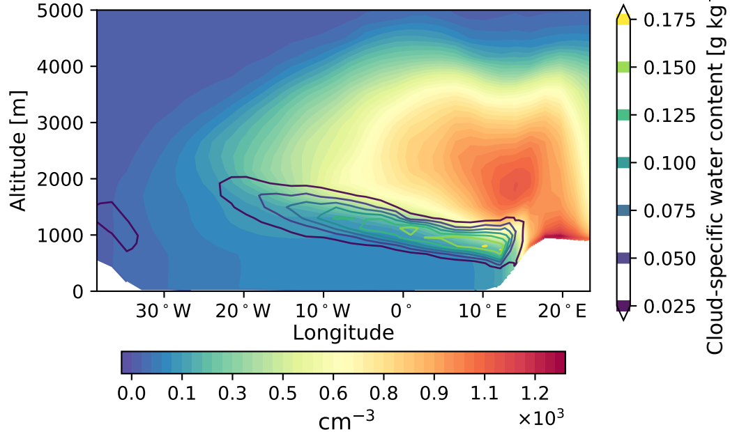
(b) Vertical distribution
