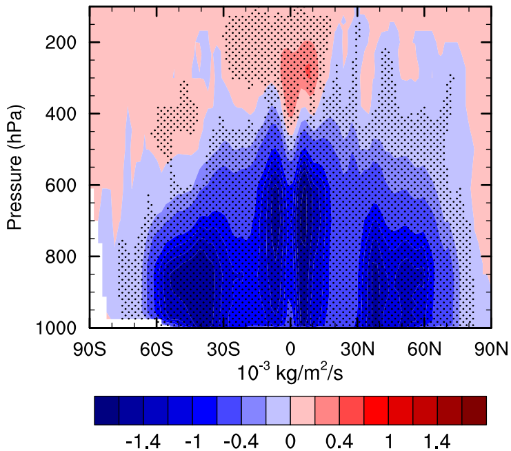
(a) Mass Flux
