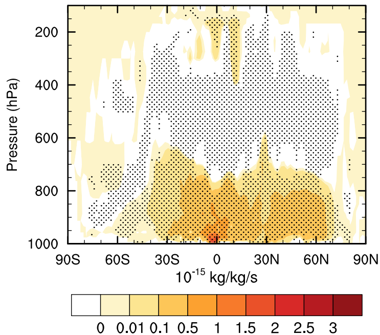
(c) Accumulation: SOA
