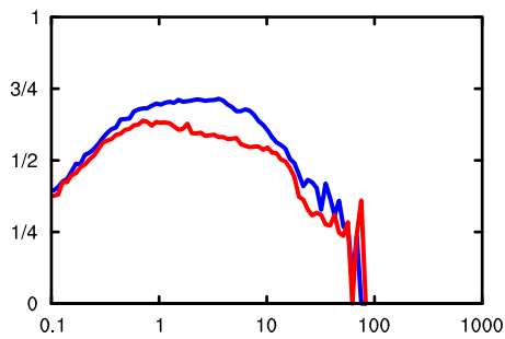
Accumulation: Sea Salt
