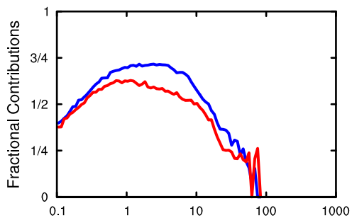
Accumulation: Black Carbon
