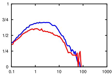
Accumulation: POM
