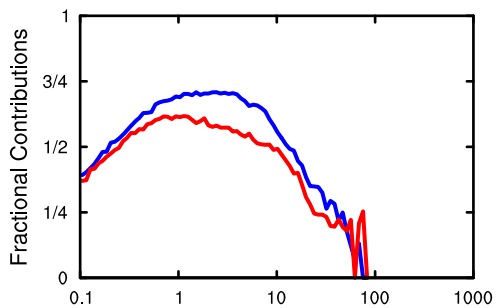
Coarse: Sulfate
