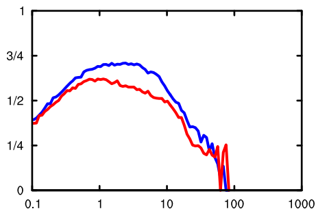
Coarse: Sea Salt
