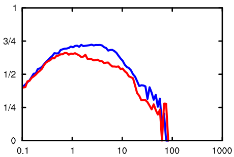
Accumulation: Dust
