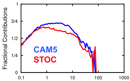
Accumulation: Sulfate
