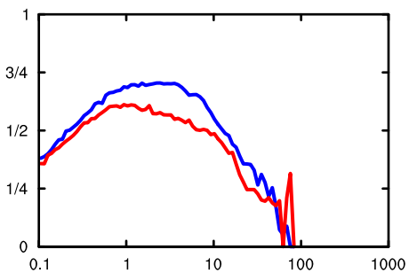
Accumulation: SOA
