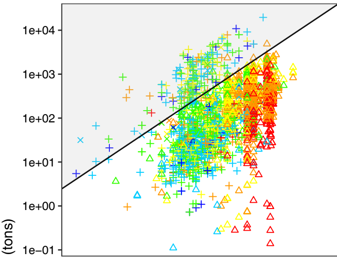
(c) NO x (2010)
