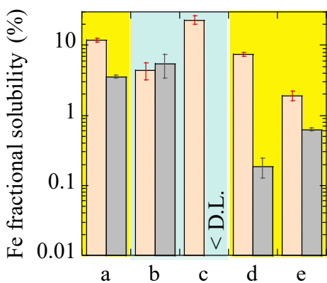
(c) fractional Fe solubility
