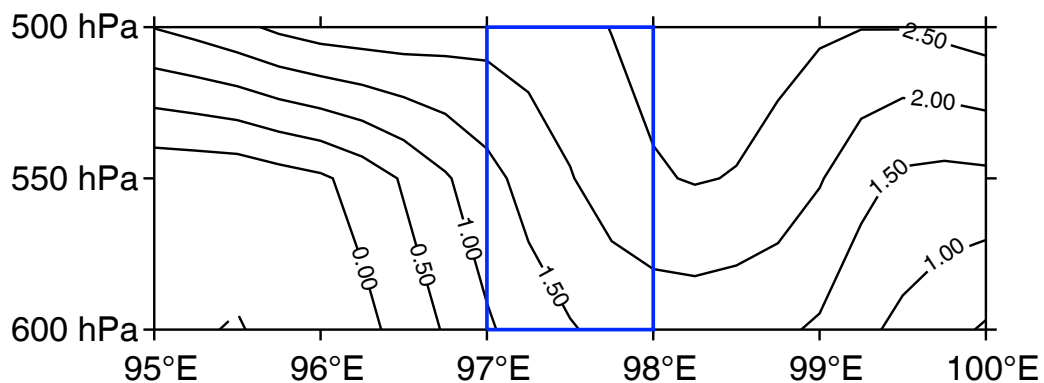
(e) 12:30 LT u (m s -1 )
