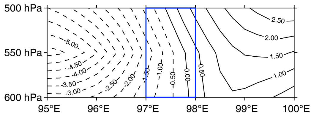
(f) 18:30 LT u (m s -1 )
