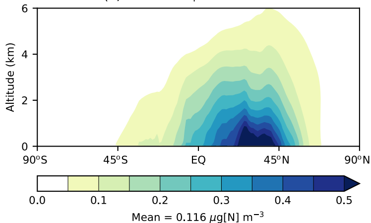
(c) SLOW: \text{NO}_3 concentration
