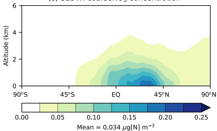
(e) SLOW: coarse \text{NO}_3 concentration
