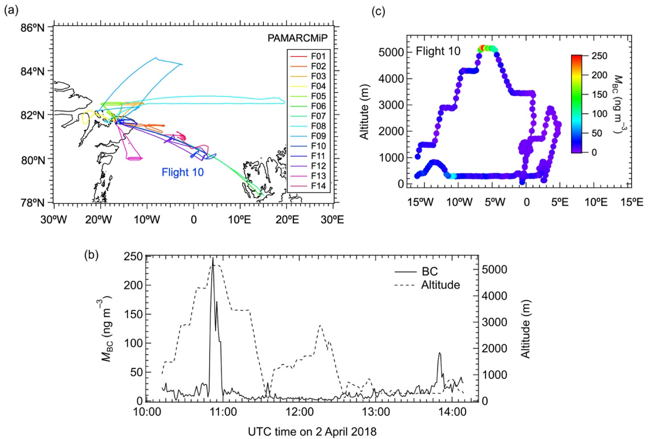
Figure S1. (a) Map of the flight tracks of the PAMARCMiP aircraft-based field experiment. (b) Time series of one-minute data of BC mass concentration ( M_{BC} ) (solid line) and aircraft altitudes (dashed line) for Flight 10 on 2 April 2018. (c) Altitude-longitude cross section of M_{BC} for the same flight. The plumes with enhanced M_{BC} values were observed at altitudes around 5 km.
