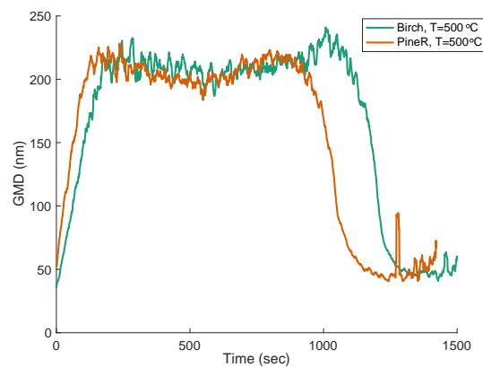
Figure S14. Geometric mean diameter (GMD) for birch and pineR at 500°C using the size distribution measured by the EEPS
