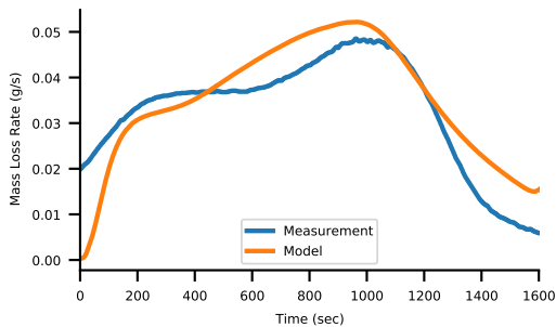
Figure S25. Gpyro modeling of mass loss rate of pineR pyrolysis at 400°C
