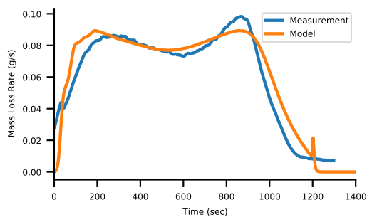
Figure S29. Gpyro modeling of mass loss rate of birch pyrolysis at 500°C
