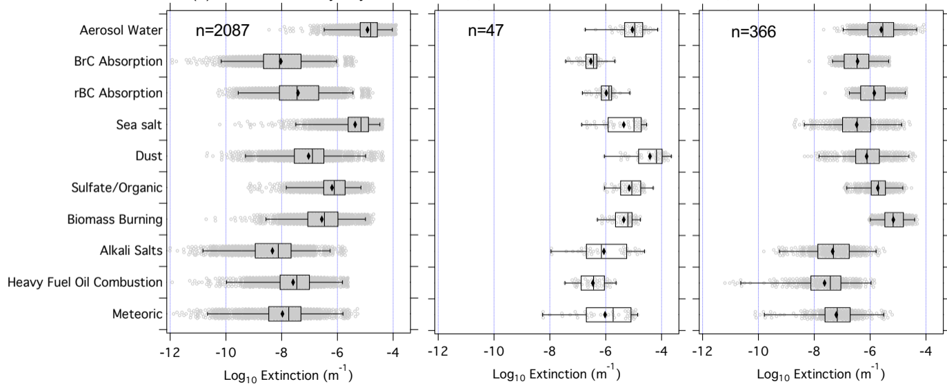
(a) Marine Boundary Layer
