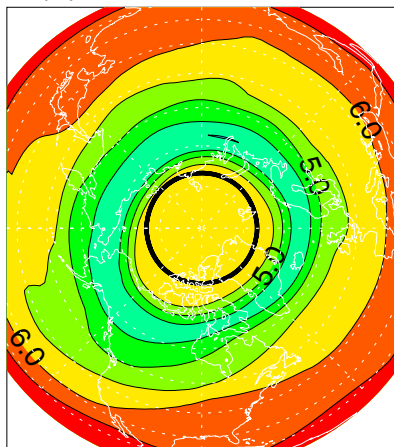
(e) Feb 15, NAVGEM
