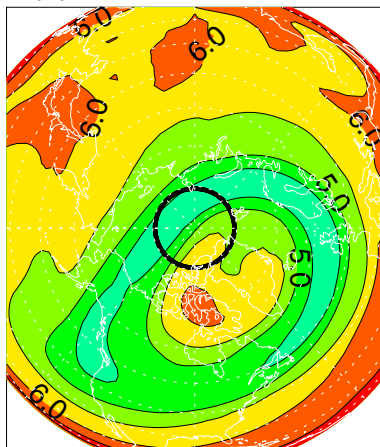
(f) Mar 1, NAVGEM
