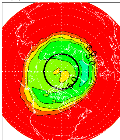
(e) Feb 15, NAVGEM
