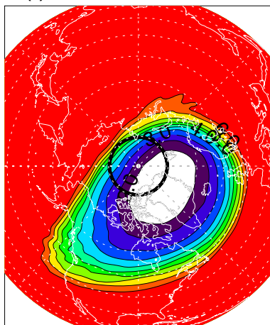
(f) Mar 1, NAVGEM
