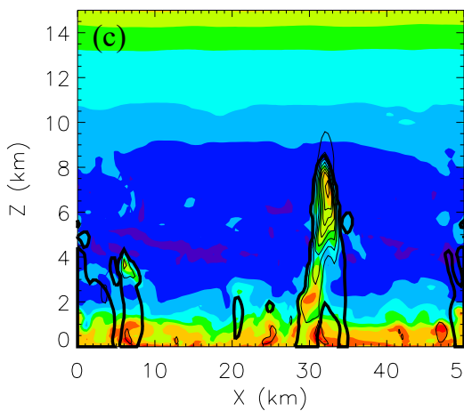
IAB X-Z Cross Section
