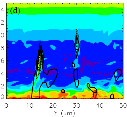
IAB Y-Z Cross Section
