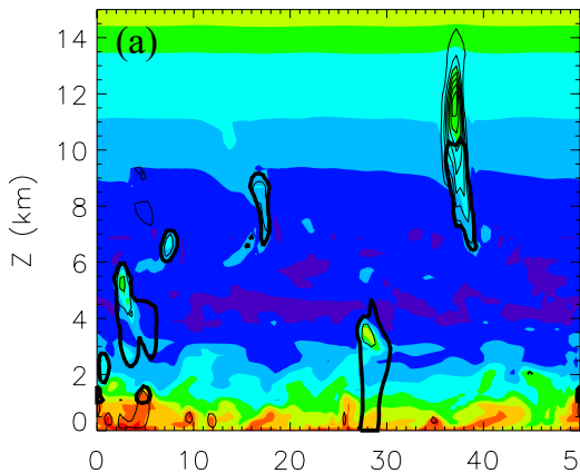
IAB X-Z Cross Section
