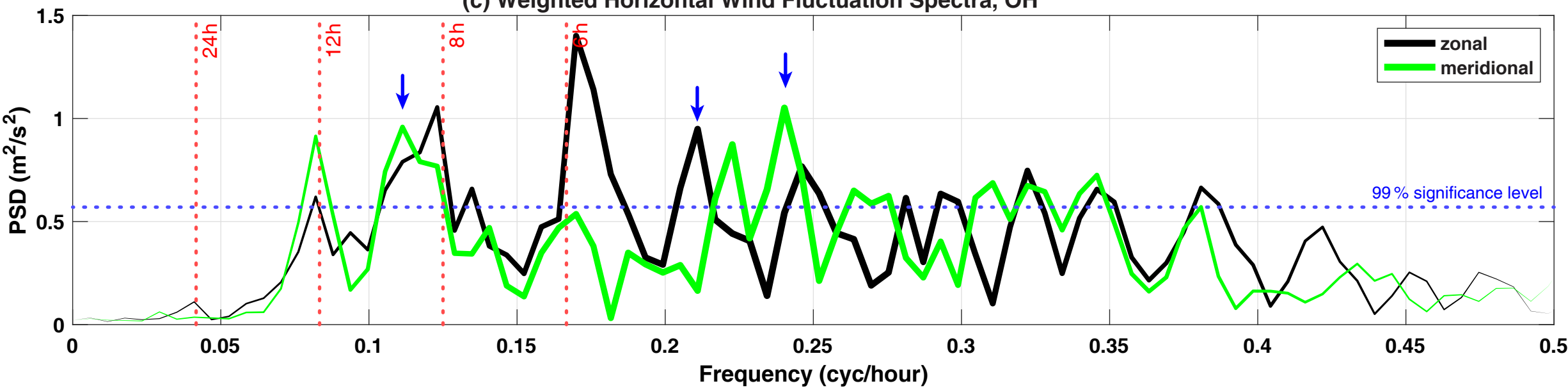
(c) Weighted Horizontal Wind Fluctuation Spectra, OH
