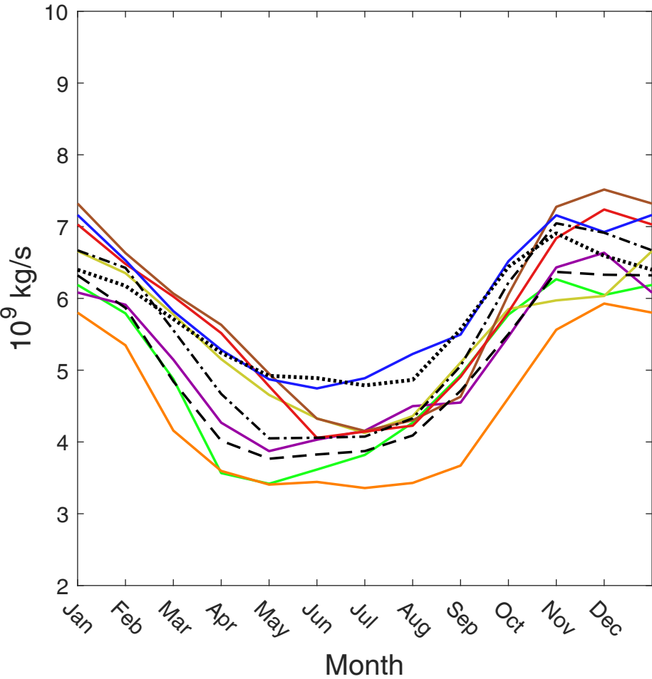
(a) Upwelling mass flux 70 hPa
