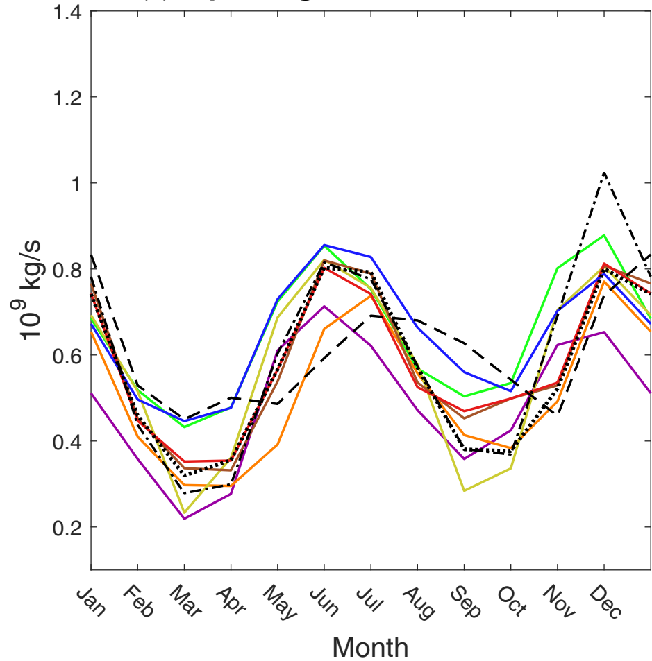
(b) Upwelling mass flux 1.5 hPa
