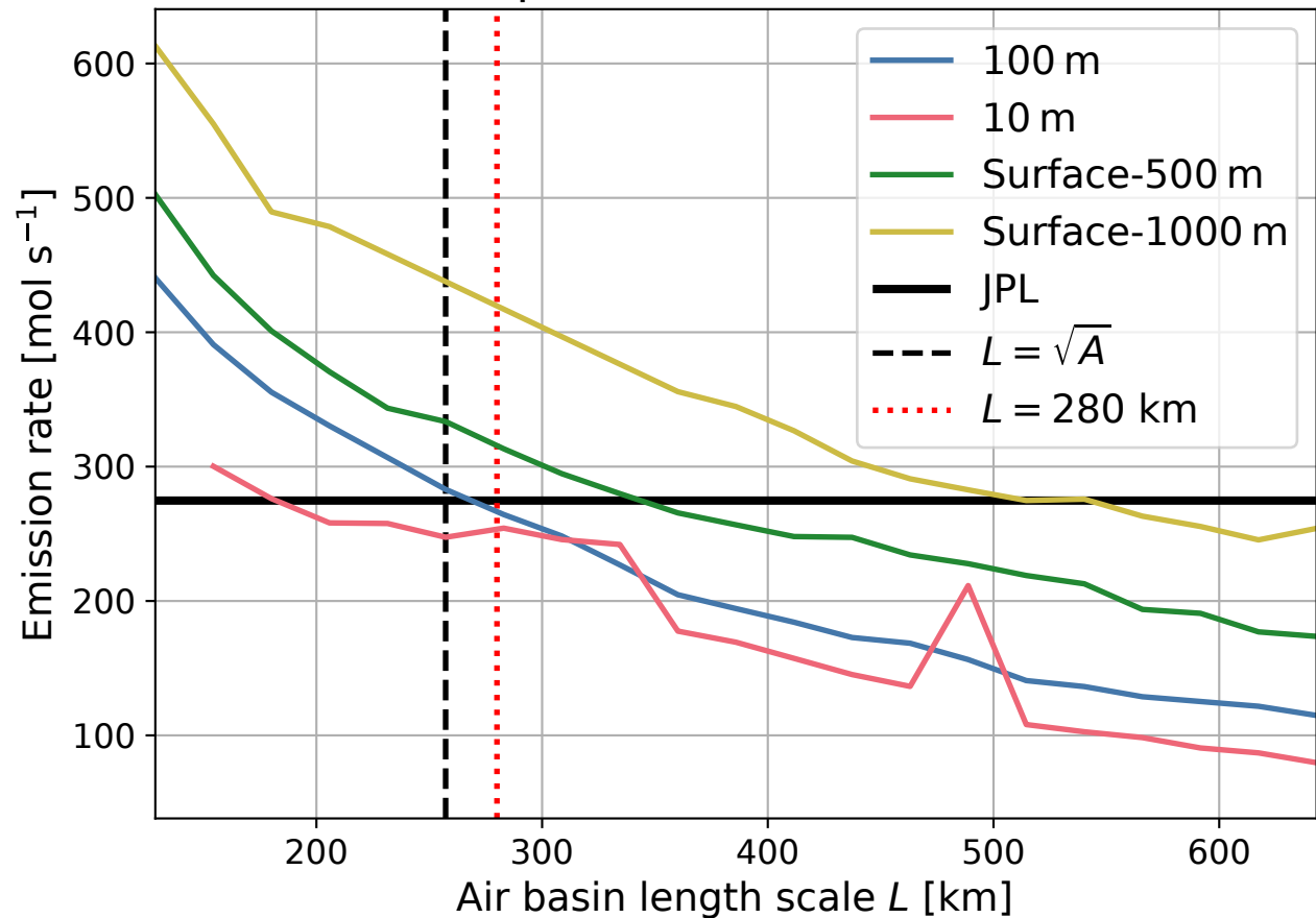
(b) Temporal mean emission rates
