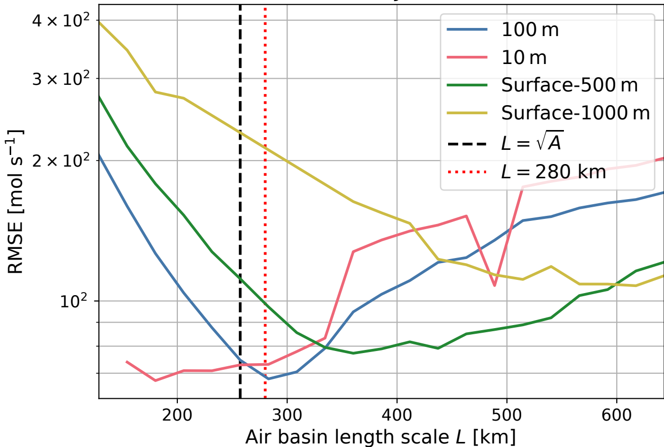
(a) RMSE relative to JPL emission rates
