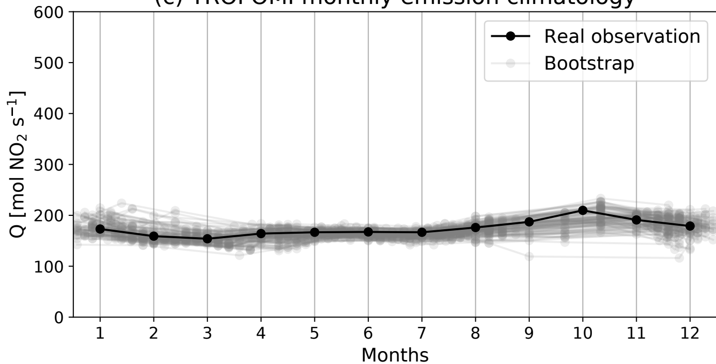
(c) TROPOMI monthly emission climatology
