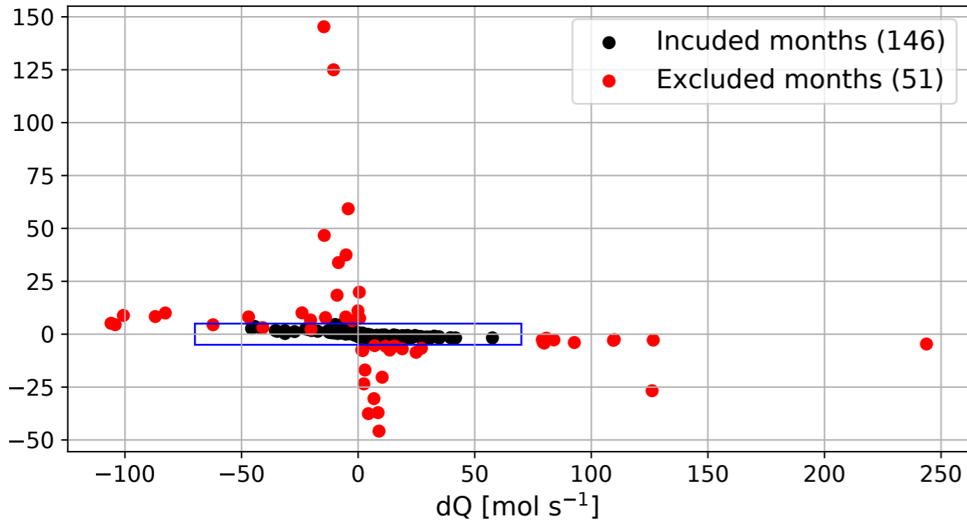
(a) OMI outlier months exclusion
