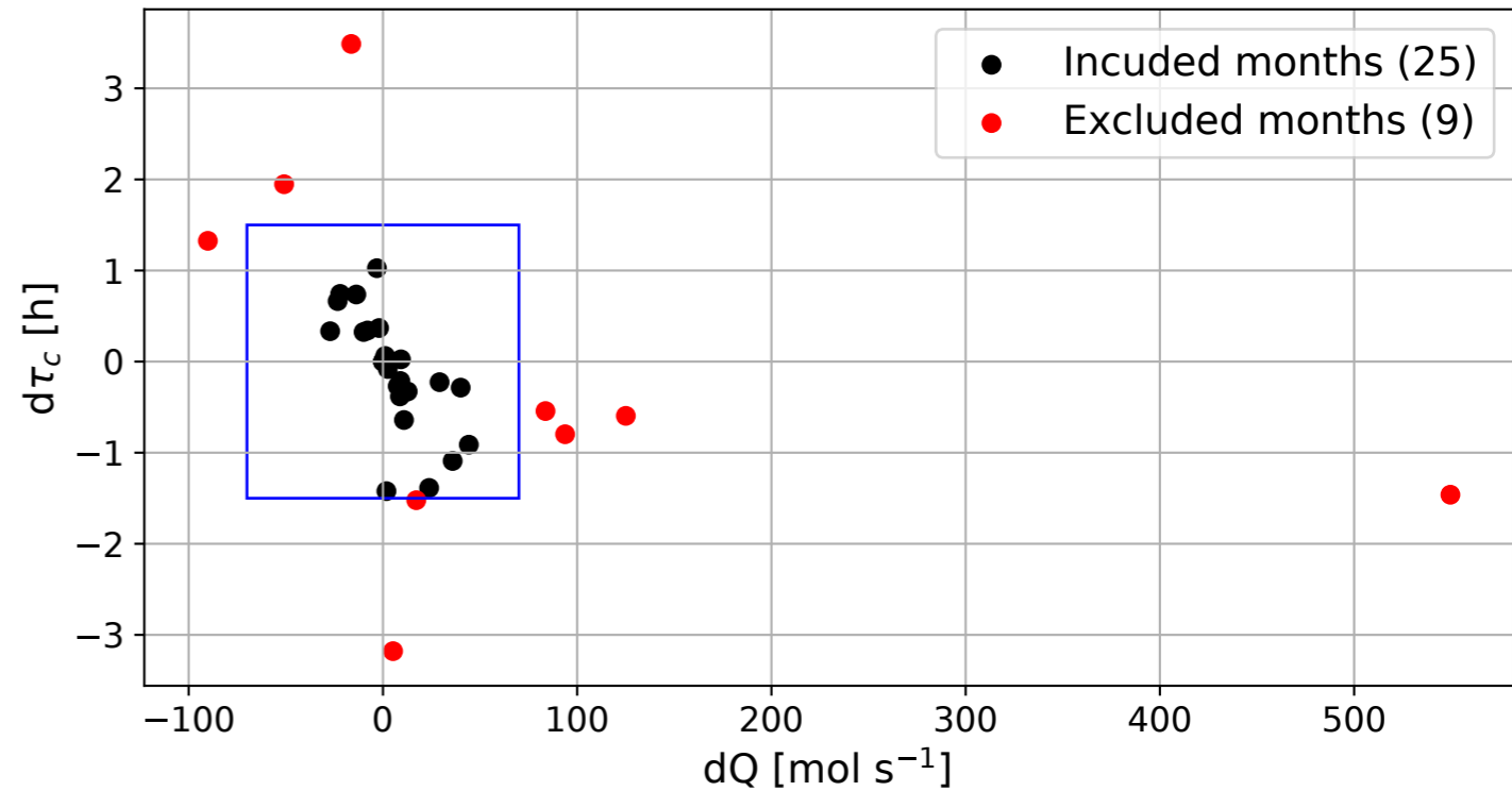
(b) TROPOMI outlier months exclusion
