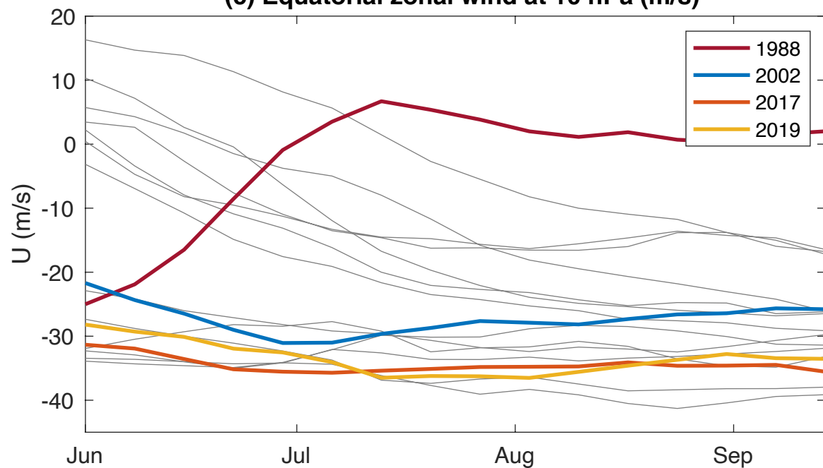
(c) Equatorial zonal wind at 10 hPa (m/s)
