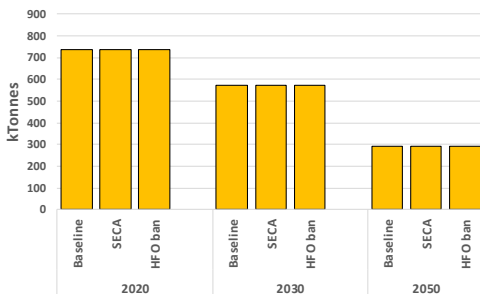
Across scenarios (HiG) - SO 2 emissions
