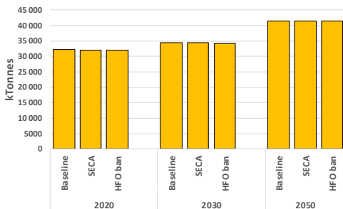
Across scenarios (BAU) - SO 2 emissions
