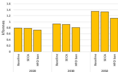
Across scenarios (HiG) - BC emissions
