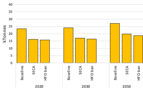
Across scenarios (BAU) - BC emissions
