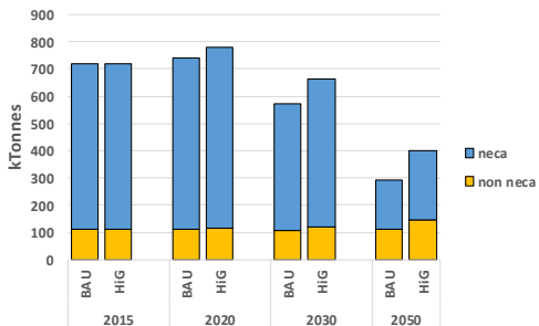
Baseline scenario - BC emissions
