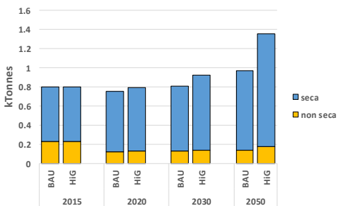
Baseline scenario - BC emissions
