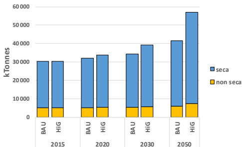
Baseline scenario - SO 2 emissions
