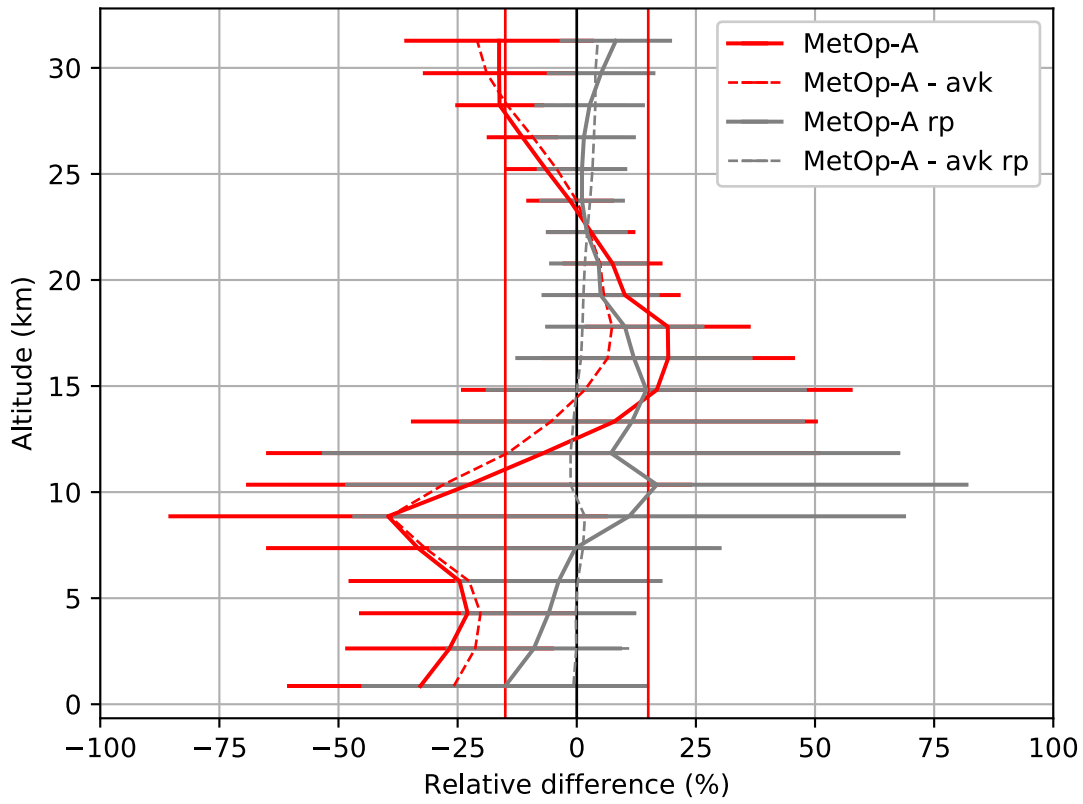
Relative difference plots for Uccle
